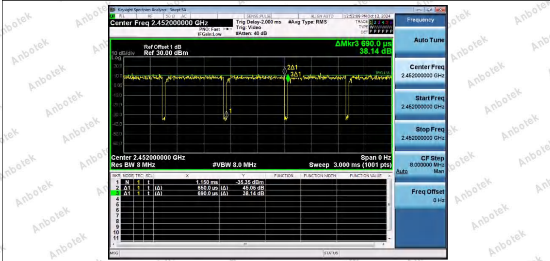
NTNV-11N40MIMO-Ant1-2452
