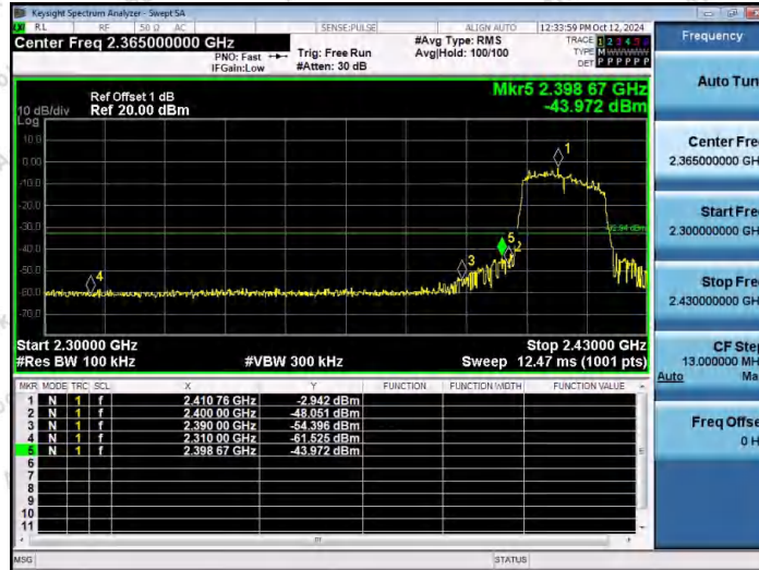
11N20MIMO-Ant2-2412-PASS
