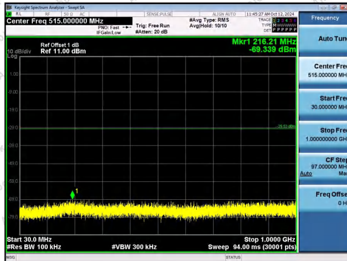
11B-Ant2-2462-30~1000-PASS
