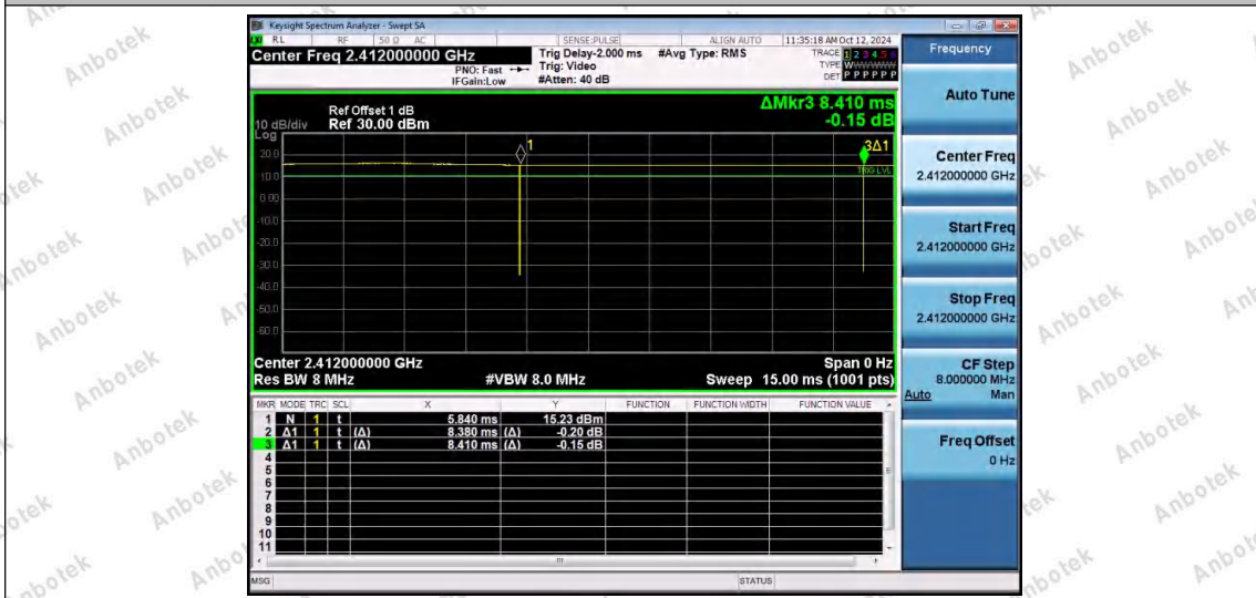
NTNV-11B-Ant2-2412
