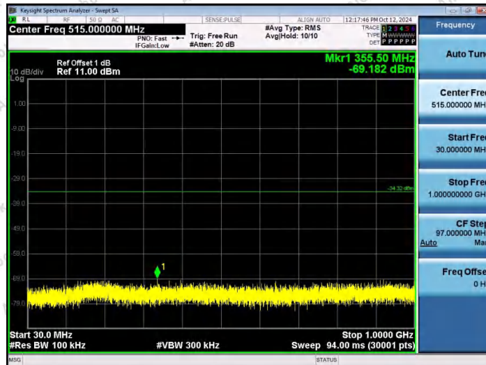
11G-Ant2-2437-30~1000-PASS
