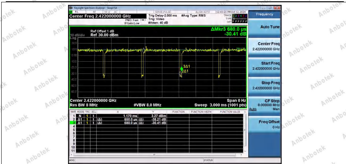
NTNV-11N40MIMO-Ant1-2422
