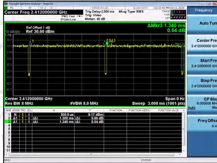
NTVN-11N20MIMO-Ant1-2412
