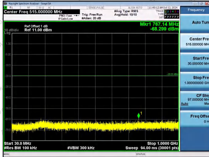
11B-Ant2-2437-30~1000-PASS
