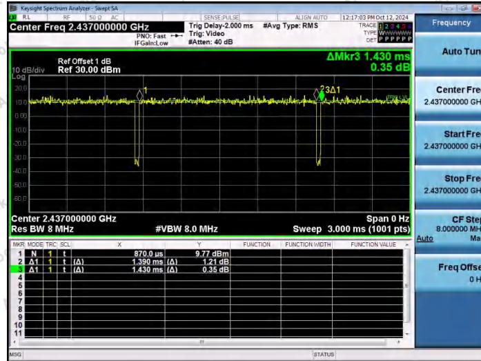
NTNV-11G-Ant2-2437
