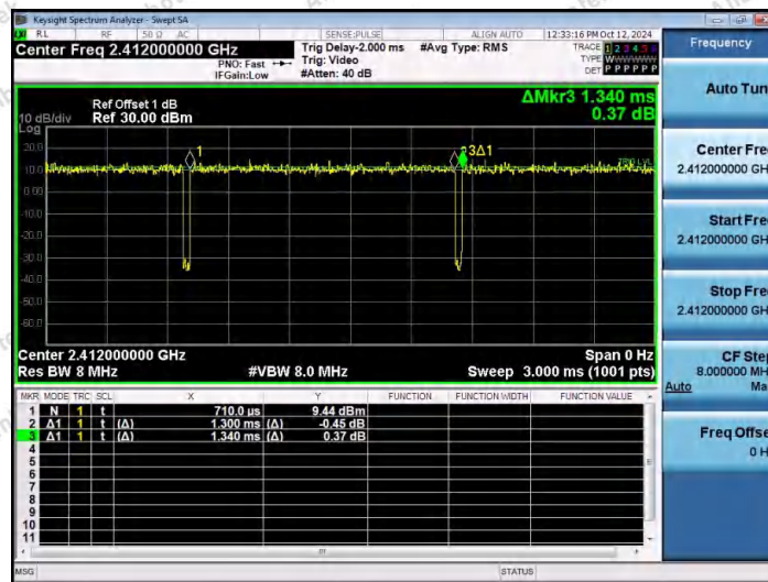
NTVN-11N20MIMO-Ant2-2412
