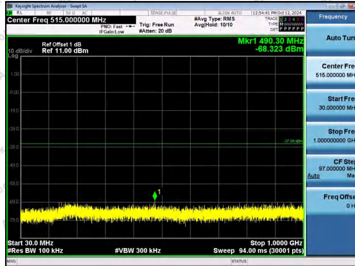
11N40MIMO-Ant2-2452-30~1000-PASS
