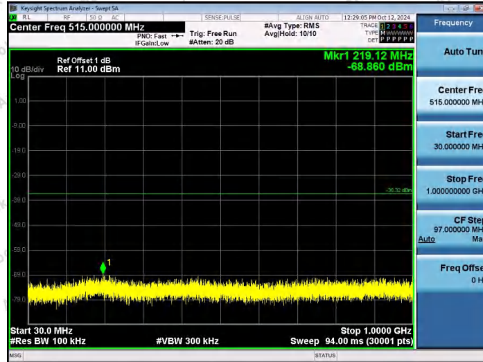
11G-Ant2-2462-30~1000-PASS
