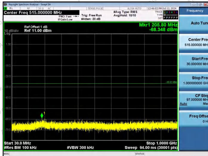
11N40MIMO-Ant2-2422-30~1000-PASS
