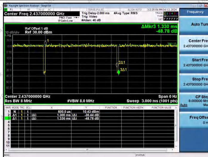
NTVN-11N20MIMO-Ant1-2437
