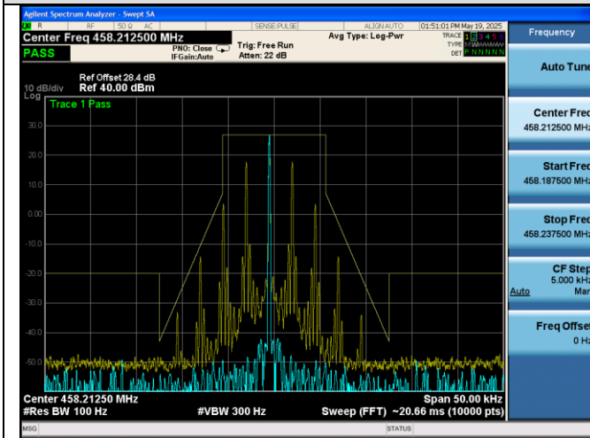
Emission Mask D@406.125MHz-2W-4FSK
