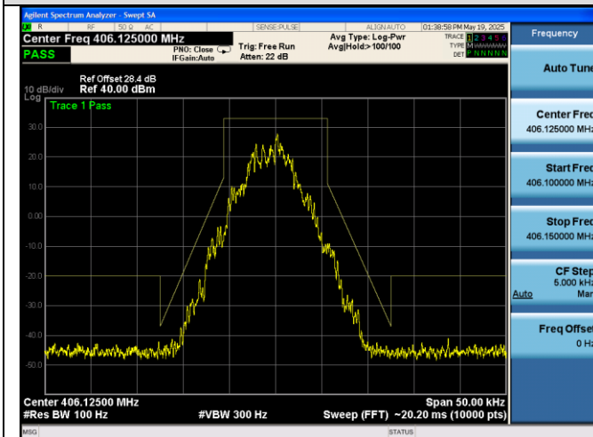
Emission Mask D@458.2125MHz-2W-4FSK
