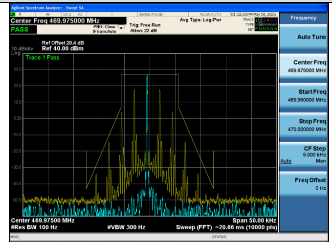
Emission Mask D@453.2125MHz-2W-4FSK
