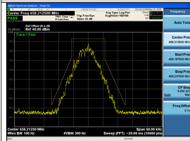
Emission Mask D@458.2125MHz-2W-4FSK
