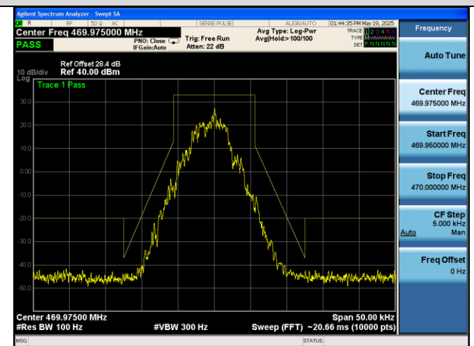
Emission Mask D@469.975MHz-2W-4FSK
