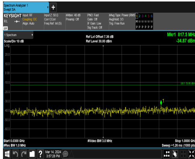
Band66-15MHz-QPSK-132322-1RB#0-Range2:1000~20000MHz
