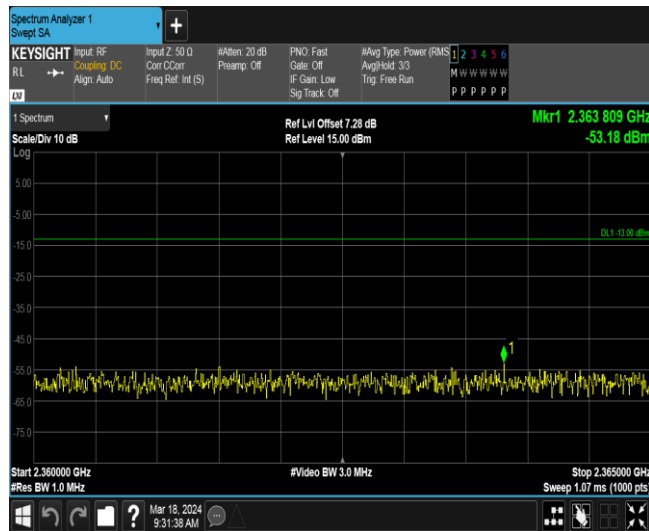
Band40-5MHz-16QAM-38725-1RB#0-Range13:2365~26500MHz
