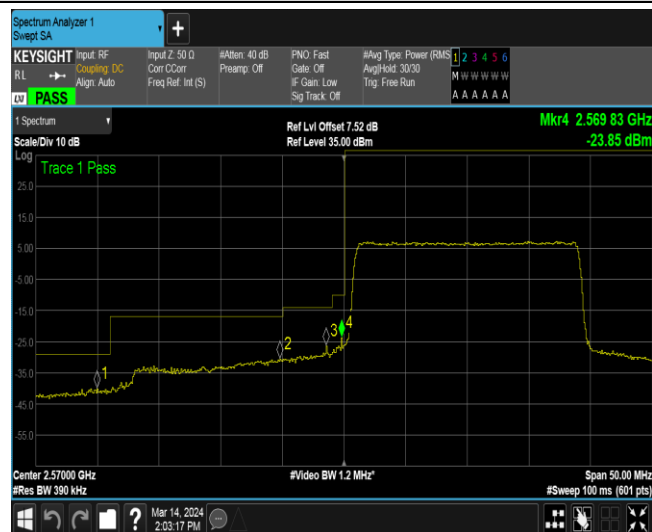
Band38-20MHz-QPSK-37850-100RB#0
