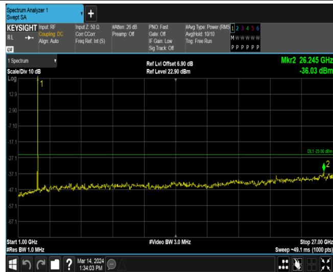
Band38-10MHz-16QAM-38200-1RB#0-Range2:1000~27000MHz
