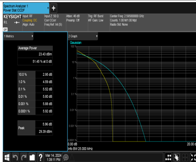
Band38-10MHz-QPSK-38000-1RB#0
