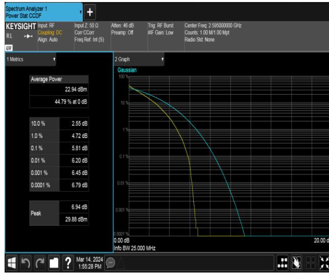
Band38-15MHz-QPSK-38175-1RB#0
