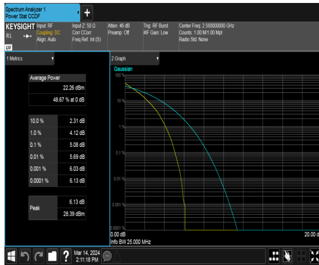
Band38-20MHz-QPSK-38000-1RB#0
