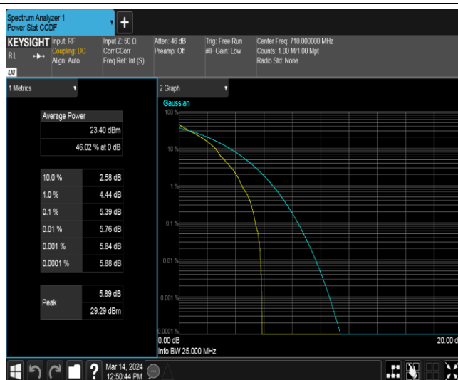
Band17-5MHz-QPSK-23790-25RB#0
