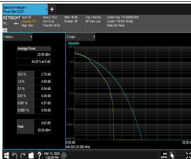
Band17-10MHz-16QAM-23790-50RB#0
