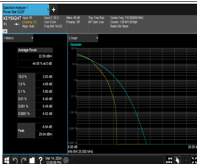
Band17-5MHz-16QAM-23790-25RB#0
