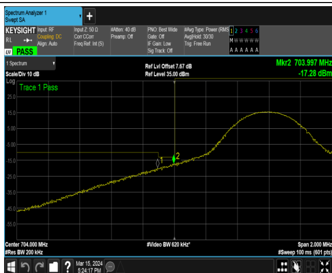
Band17-10MHz-QPSK-23780-1RB#49
