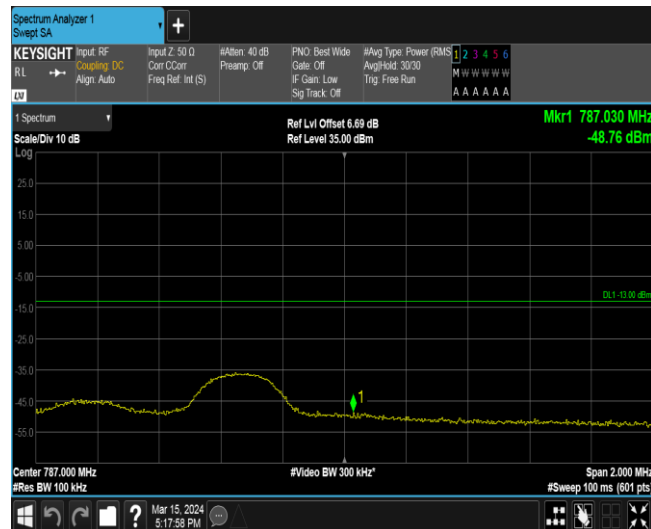
Band13-5MHz-QPSK-23255-1RB#24
