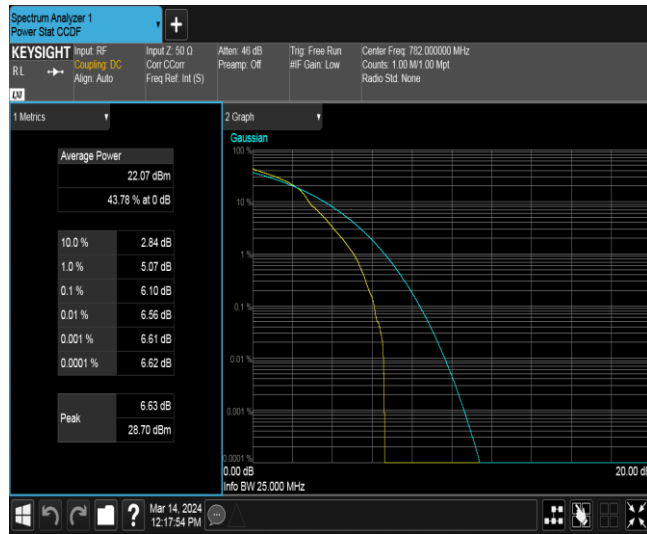
Band13-5MHz-16QAM-23230-25RB#0
