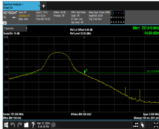
Band13-5MHz-QPSK-23255-25RB#0
