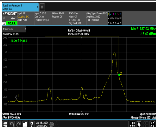
Band13-10MHz-QPSK-23230-50RB#0
