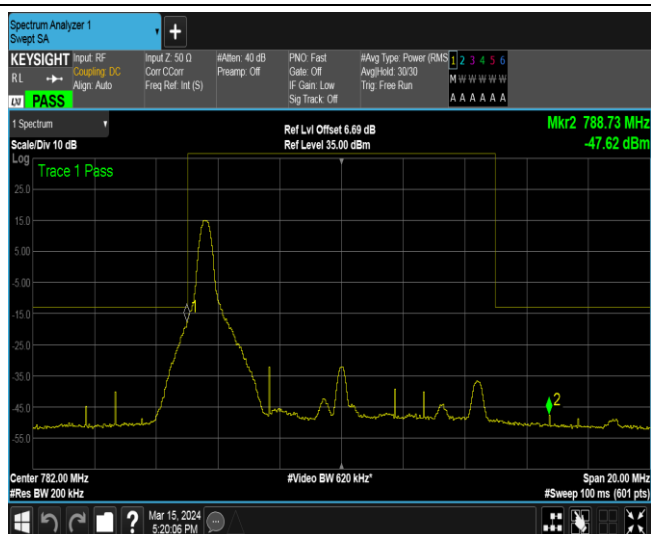
Band13-10MHz-QPSK-23230-1RB#49
