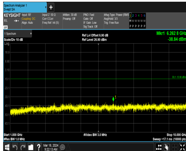
Band13-5MHz-QPSK-23255-1RB#0-Range3:1559~1610MHz
