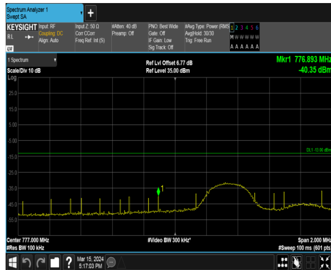
Band13-5MHz-QPSK-23205-25RB#0
