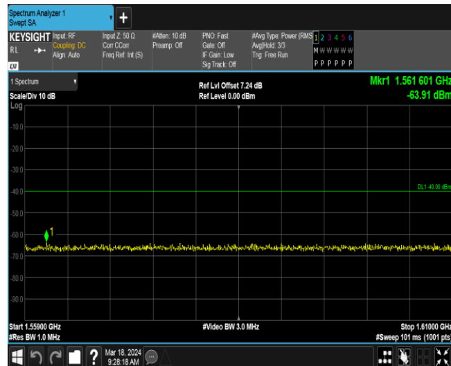
Band13-10MHz-16QAM-23230-1RB#0-Range3:1559~1610MHz
