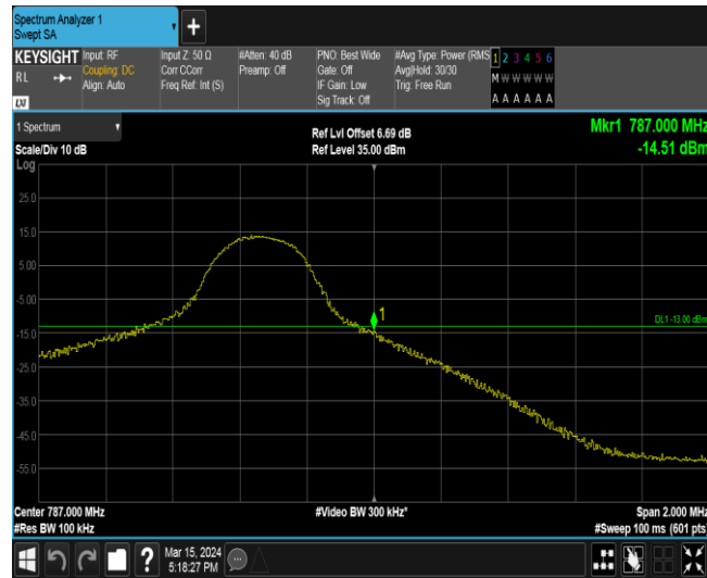
Band13-5MHz-16QAM-23255-25RB#0
