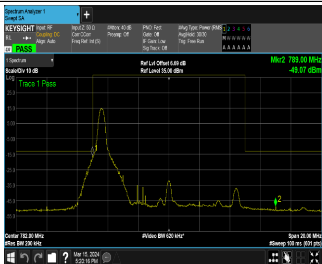
Band13-10MHz-16QAM-23230-1RB#49
