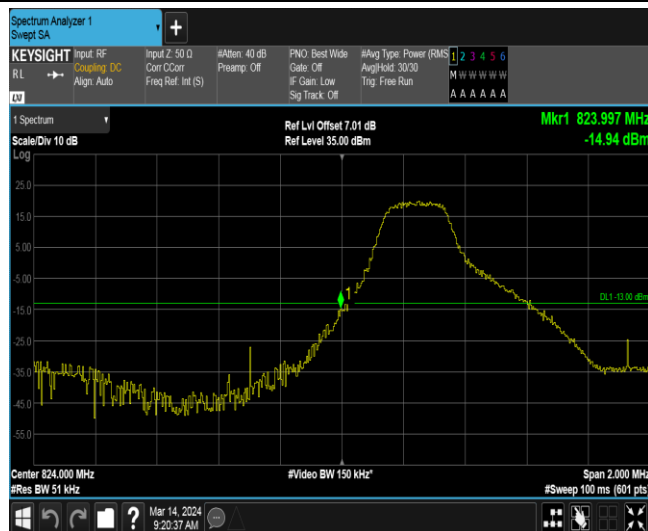
Band5-3MHz-16QAM-20415-1RB#14
