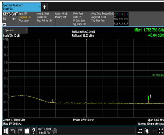
Band4-15MHz-16QAM-20325-1RB#74
