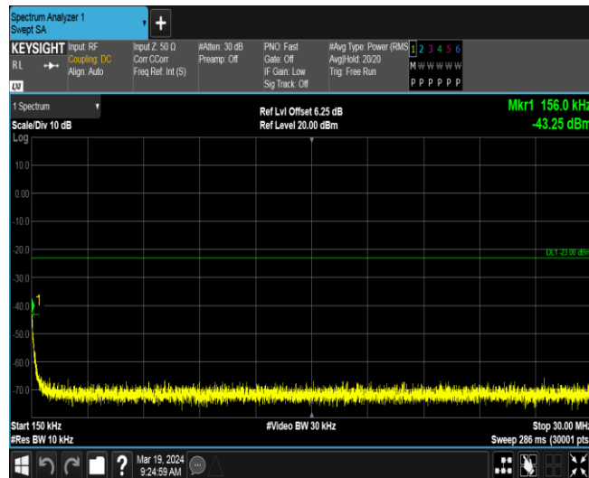
Band4-1513-5-0.15~30MHz
