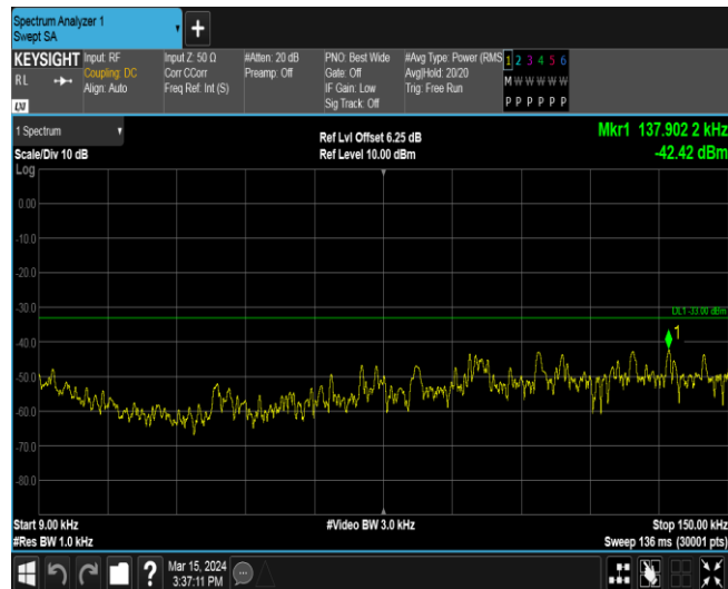
Band5-4182-2-0.009~0.15MHz
