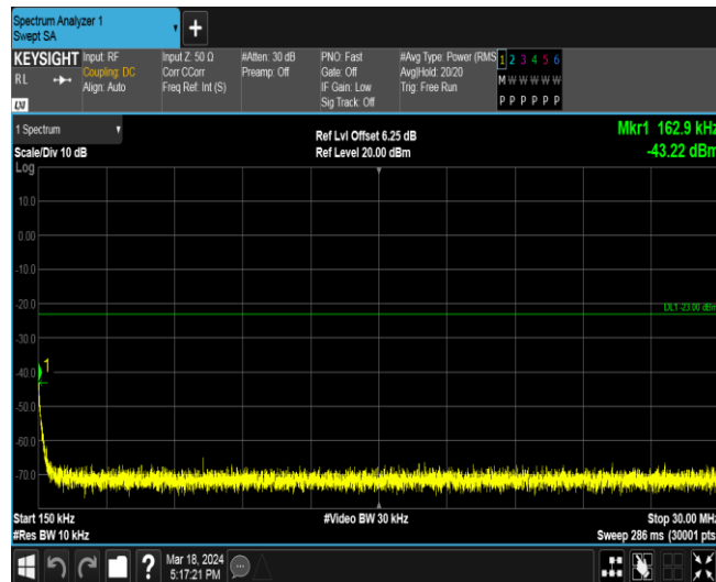
Band2-9400-5-0.15~30MHz
