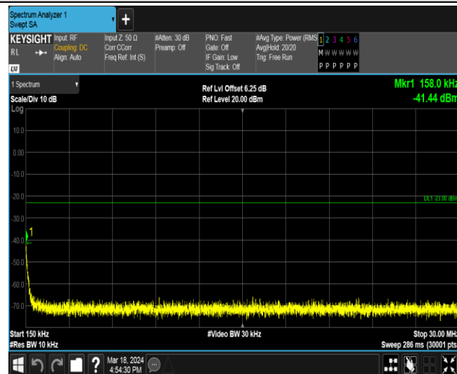
Band2-9400-4-0.15~30MHz
