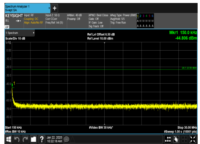
GPRS850-190-5-0.15~30MHz-PASS
