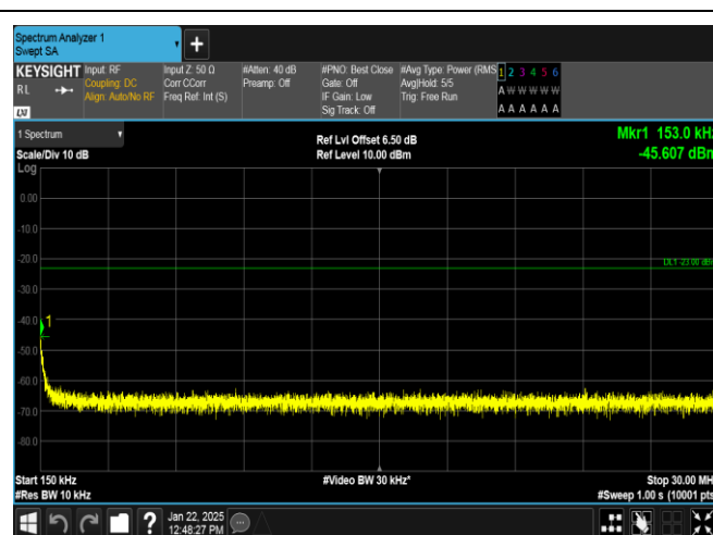
EGPRS850-190-8-0.15~30MHz-PASS
