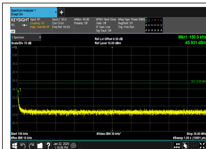
EGPRS1900-512-2-0.15~30MHz-PASS
