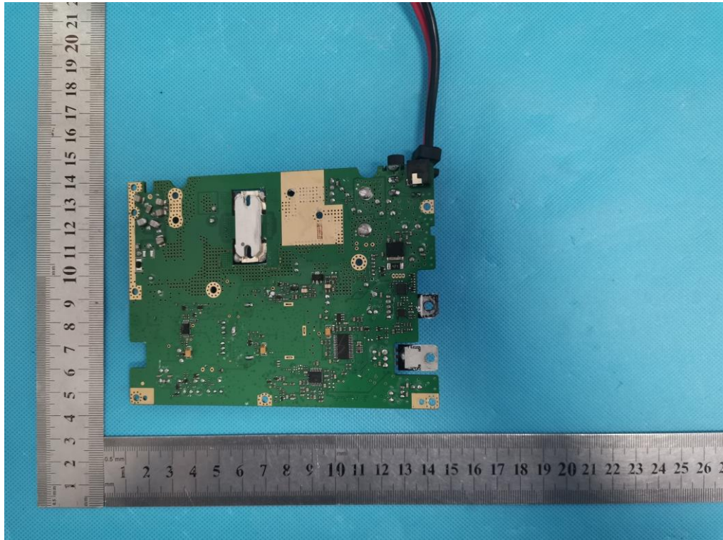
INTERNAL VIEW OF EUT(FIGURE 17)
