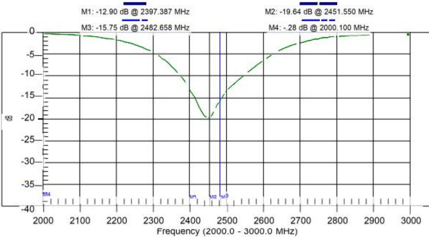
Return Loss
