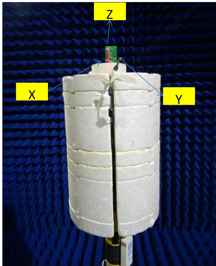
Testing environment
