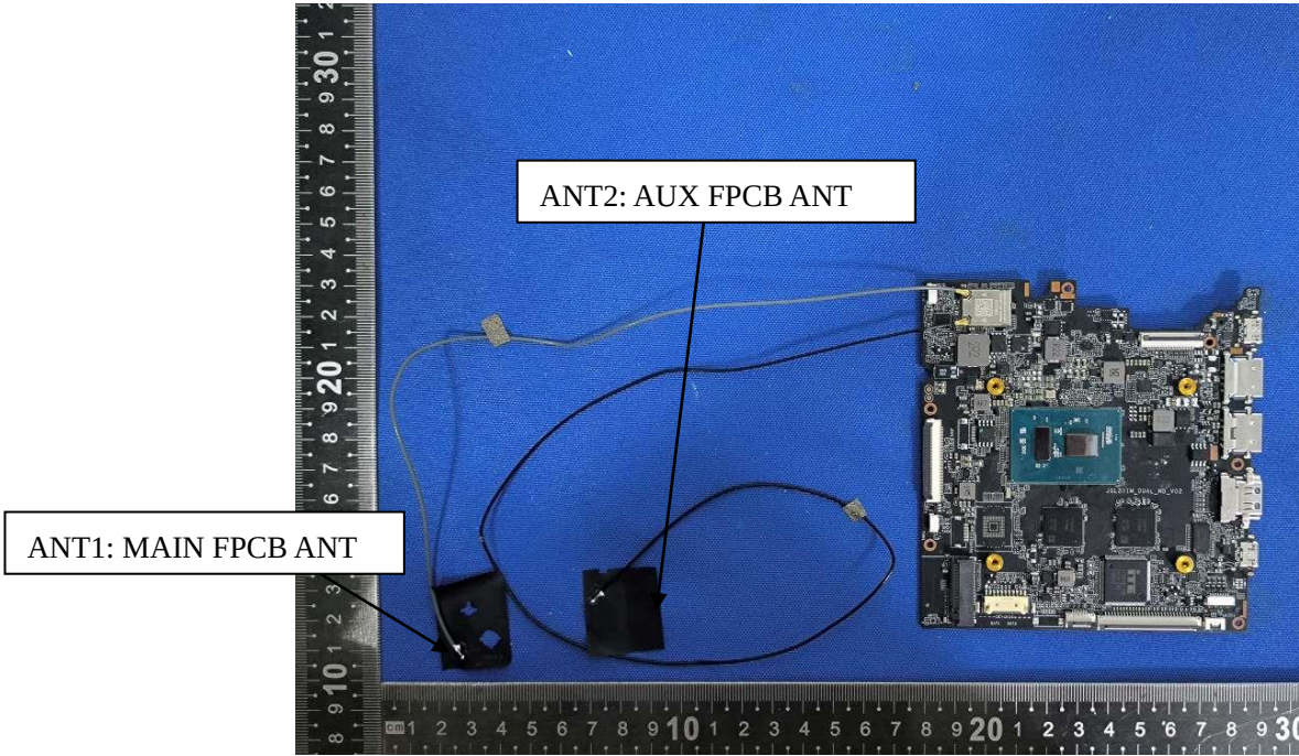
EUT Internal View 3
