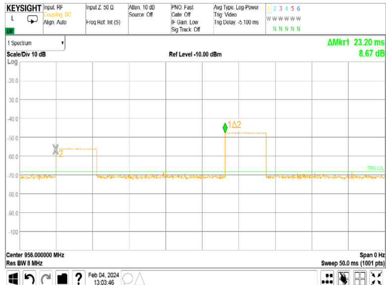
Plot 7.1.3 Transmission period at 956 MHz
