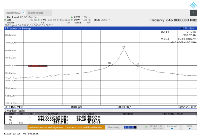
Plot 7.3.2 Occupied bandwidth test result at the fundamental frequency 646 MHz
