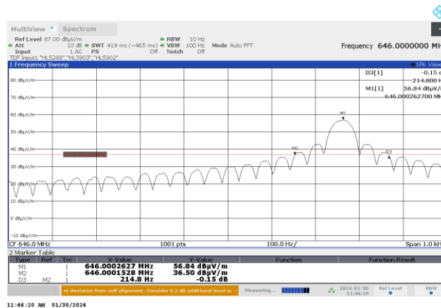
Plot 7.3.2 Occupied bandwidth test result at the fundamental frequency 646 MHz
