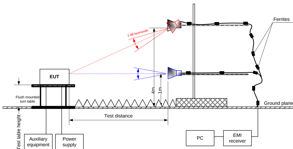
Figure 8.1.2 Setup for radiated emission measurements in 1000 – 6000 MHz range, table-top EUT
