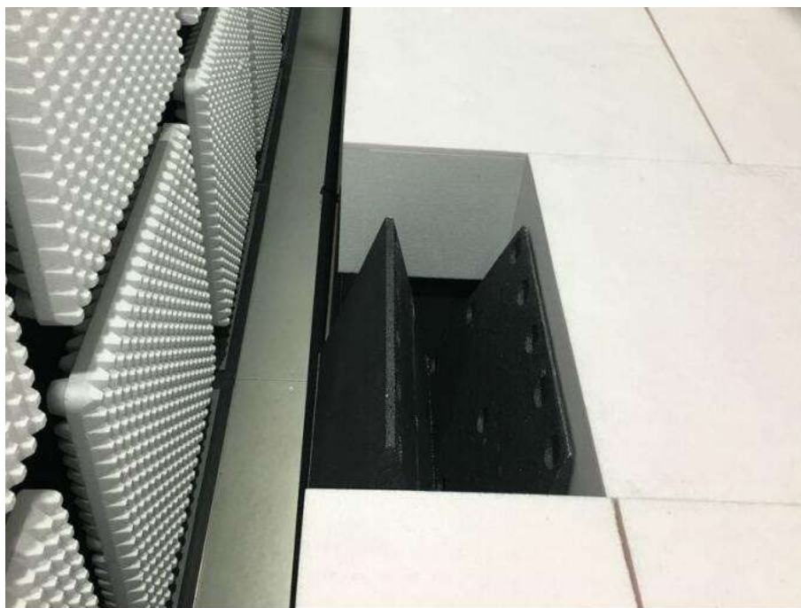
Radiated spurious emission Test Setup (Above 1GHz) There are absorbing materials under the ground.
