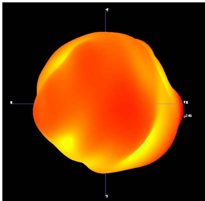
B1.3 3D Pattern for 2483.5MHz
