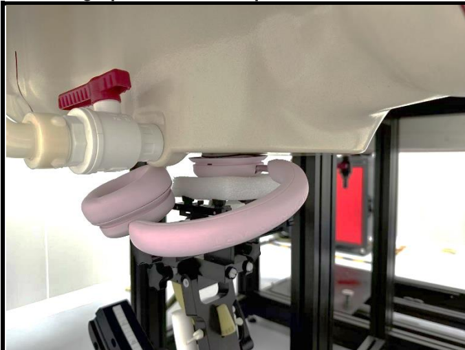
Inside of Headset_1 with 0 cm Gap
