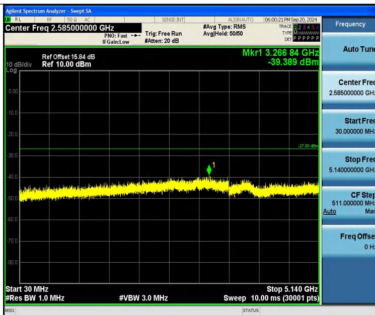
11AC20SISO-Ant1-5200-30~5140-PASS
