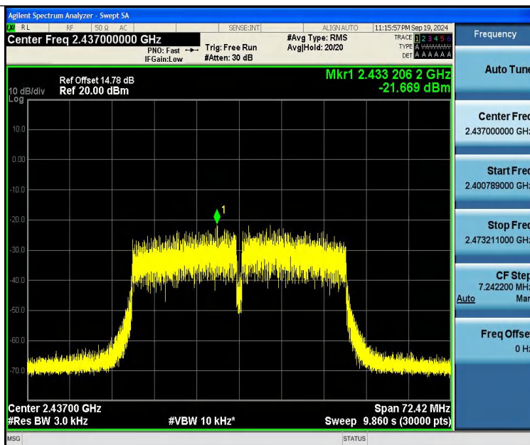
11N40SISO-Ant2-2437-PASS
