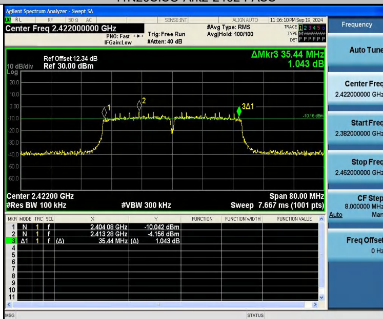
11N40SISO-Ant2-2422-PASS
