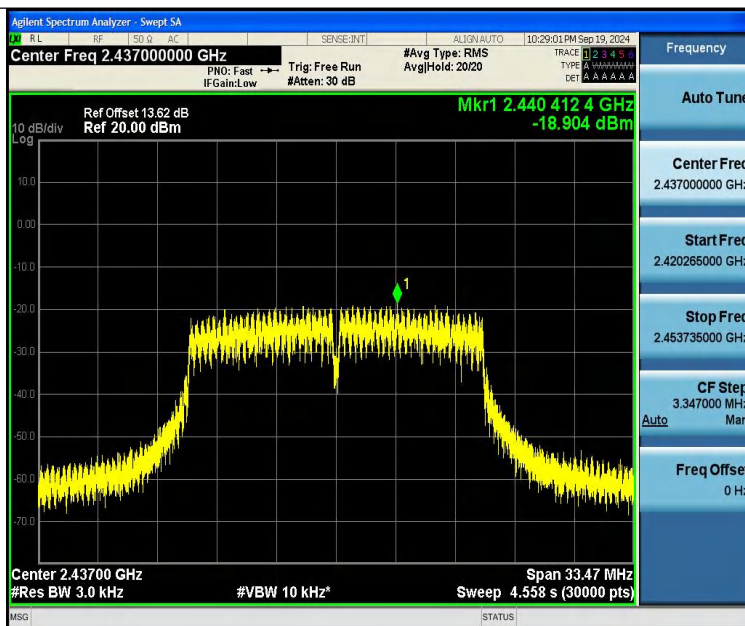
11G-Ant2-2437-PASS
