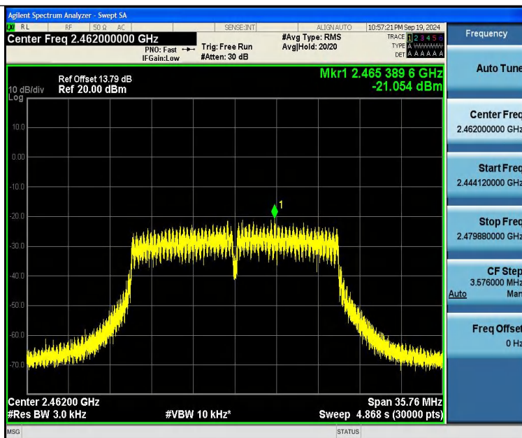
11N20SISO-Ant2-2462-PASS
