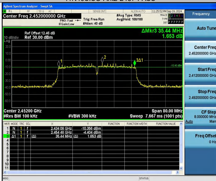
11N40SISO-Ant2-2452-PASS
