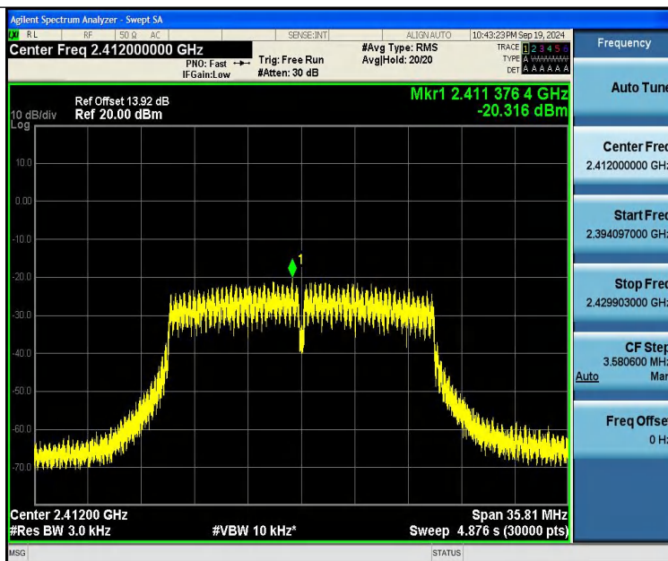
11N20SISO-Ant2-2412-PASS
