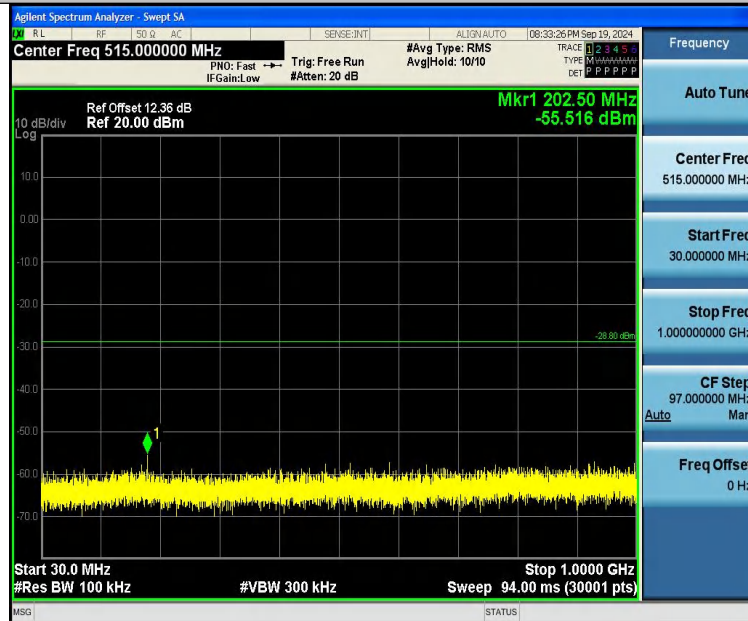
11B-Ant1-2462-30~1000-PASS
