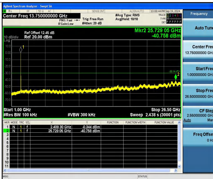
11B-Ant2-2412-1000~26500-PASS
