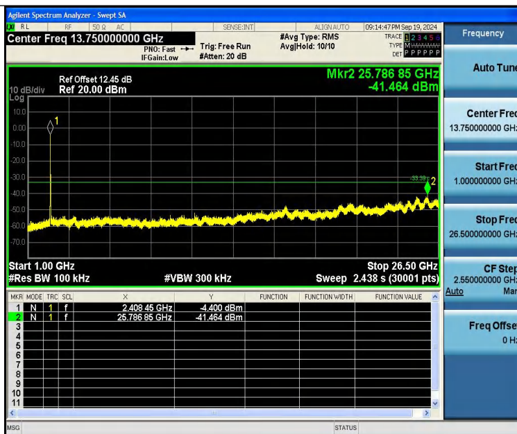
11N20SISO-Ant1-2412-1000~26500-PASS
