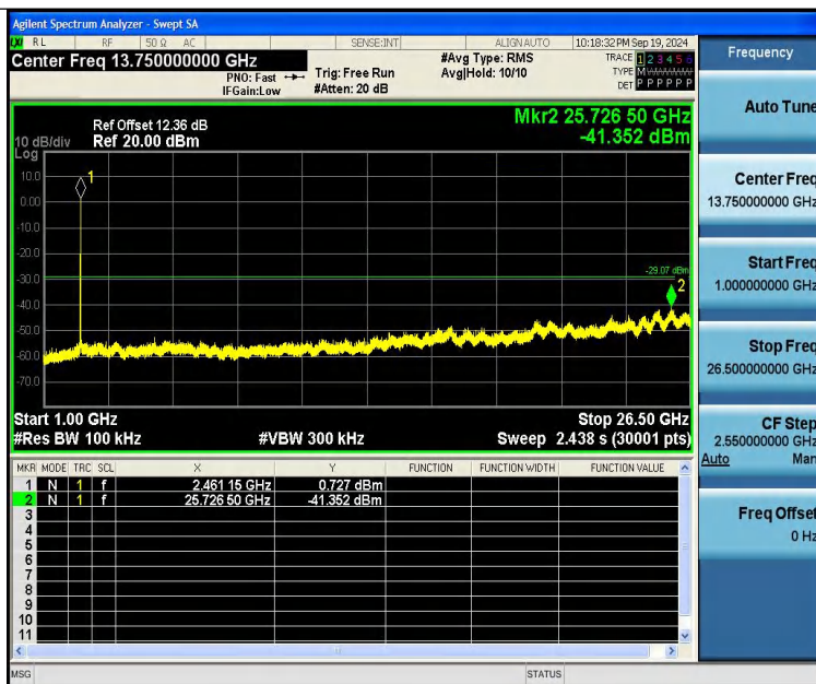
11B-Ant2-2462-1000~26500-PASS
