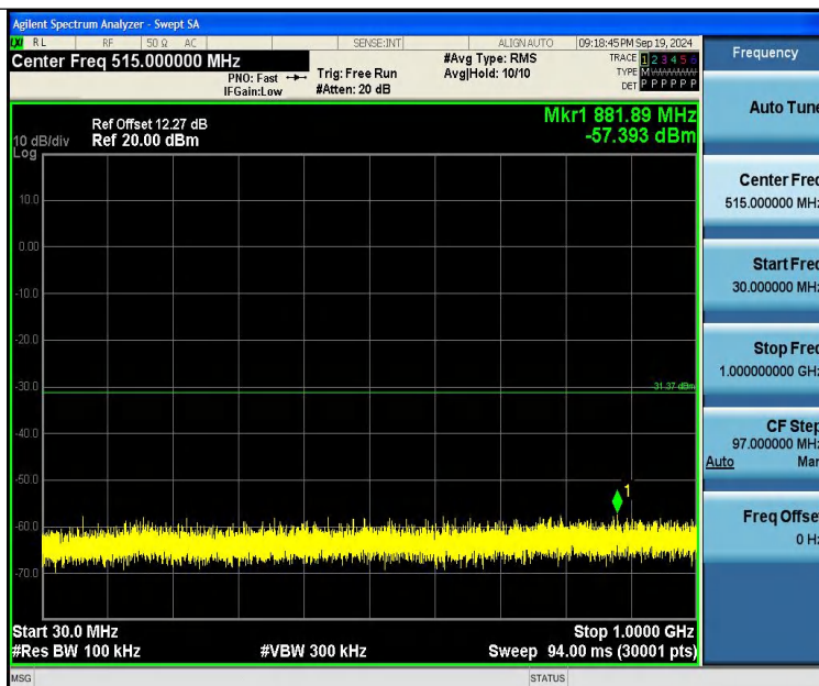
11N20SISO-Ant1-2437-30~1000-PASS
