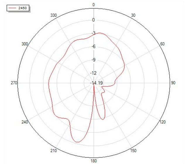
Phi=0 freq=2450MHz
