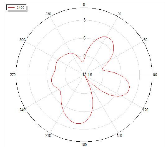
Theta=90 freq=2450MHz
