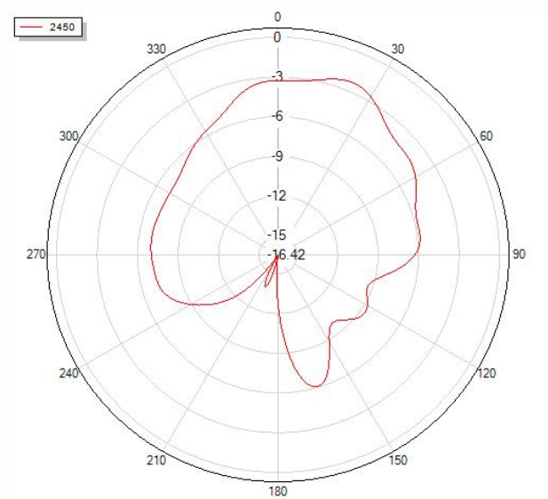
Phi=90 freq=2450MHz
