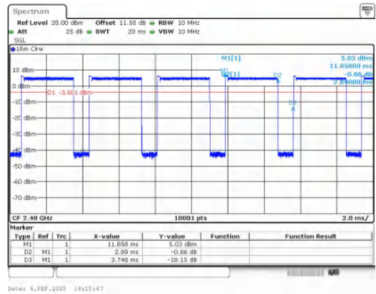
π/4DQPSK(2-DH5)_Channel 78
