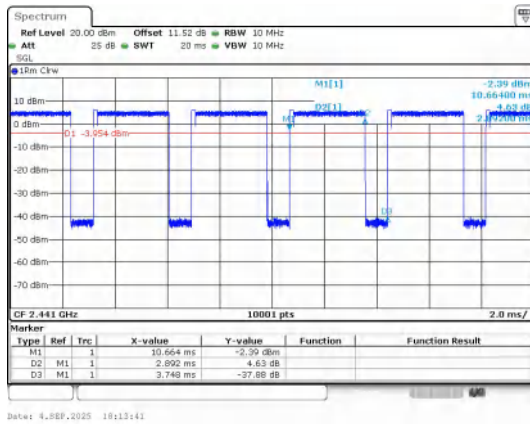
π/4DQPSK(2-DH5)_Channel 39
