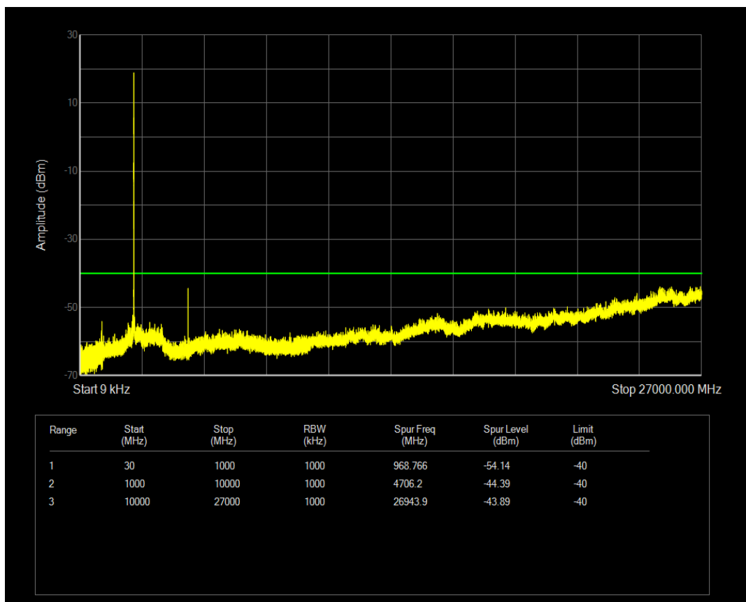
Band40(2350-2360) QPSK BW=5MHz Channel=39200 RB Size=25 Position=#0
