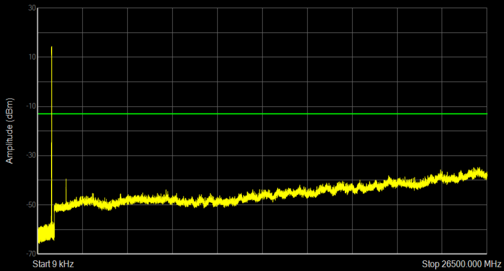
Band26b 16QAM BW=5MHz Channel=27015 RB Size=25 Position=#0
