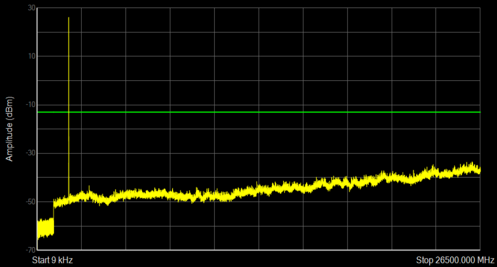
Band25 16QAM BW=10MHz Channel=26640 RB Size=1 Position=#0
