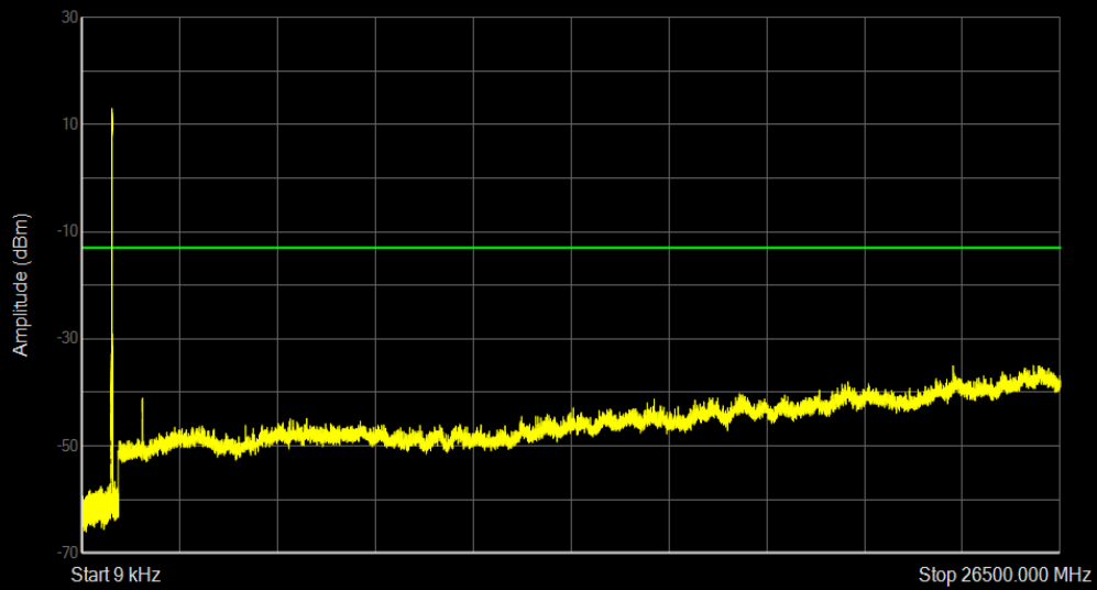
Band26b 16QAM BW=10MHz Channel=26840 RB Size=50 Position=#0
