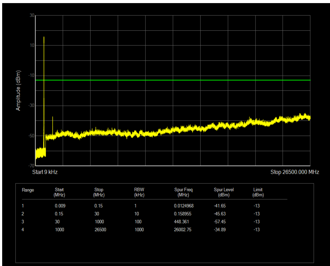
Band26b 16QAM BW=5MHz Channel=26915 RB Size=1 Position=#0
