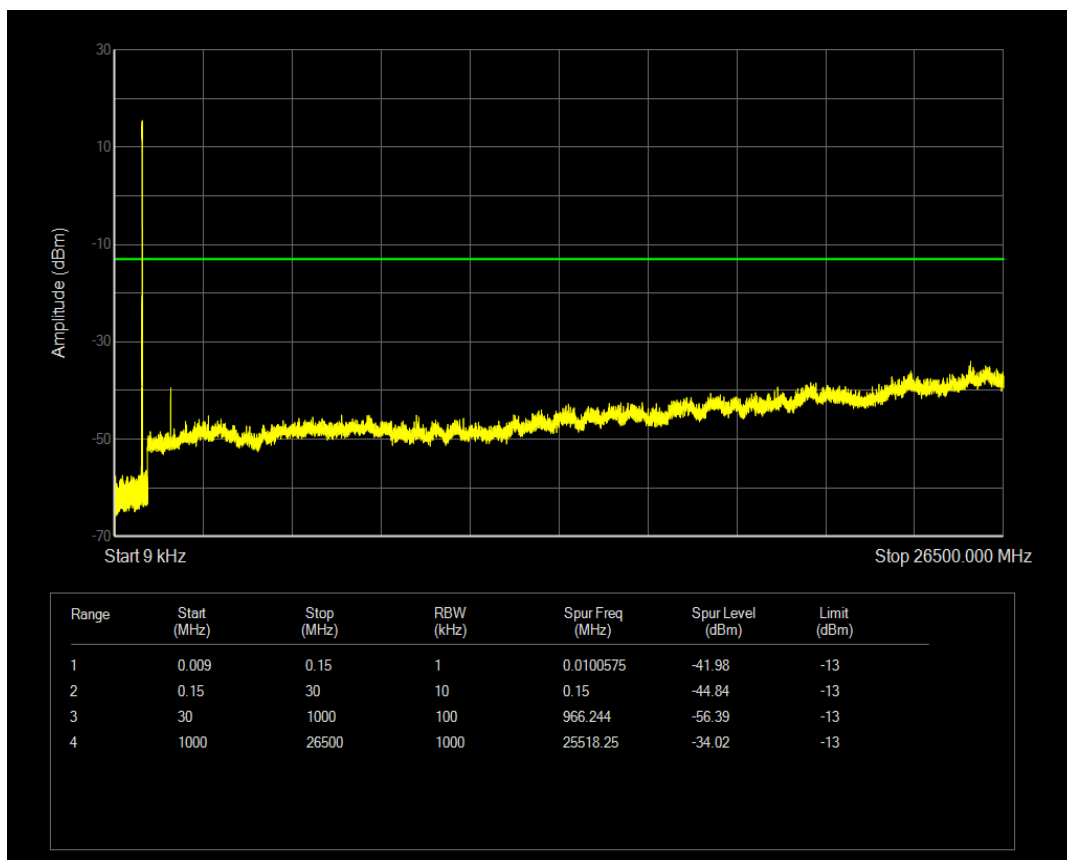
Band26b 16QAM BW=5MHz Channel=27015 RB Size=1 Position=#0
