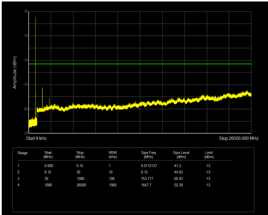
Band26b 16QAM BW=1.4MHz Channel=26797 RB Size=6 Position=#0
