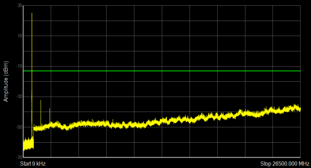
Band26b 16QAM BW=3MHz Channel=27025 RB Size=1 Position=#0
