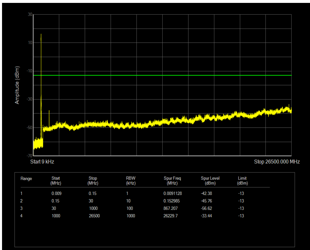
Band26a 16QAM BW=5MHz Channel=26765 RB Size=1 Position=#0
