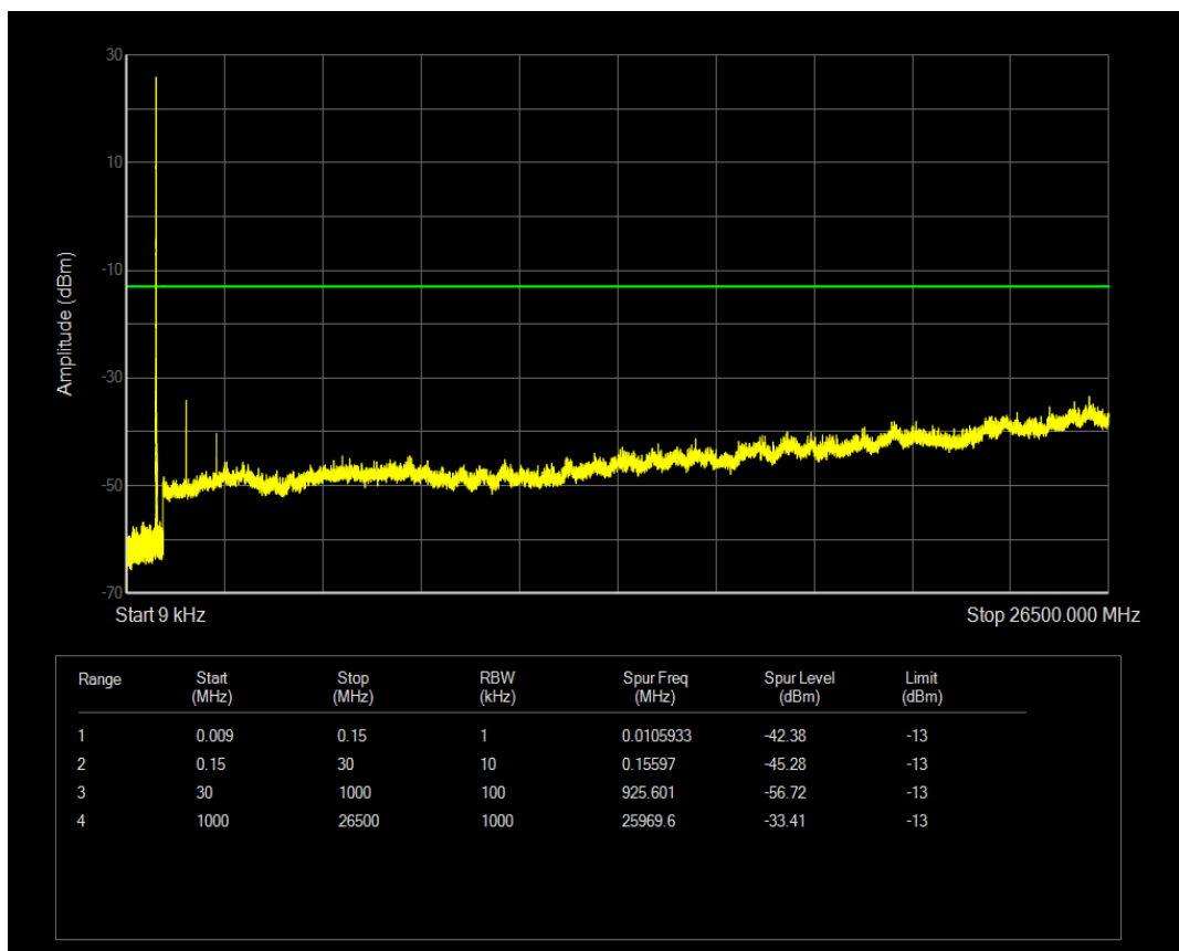
Band26a 16QAM BW=10MHz Channel=26740 RB Size=50 Position=#0
