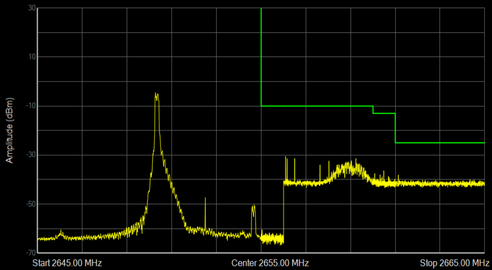
Band41 16QAM BW=5MHz Channel=41215 RB Size=1 Position=#0
