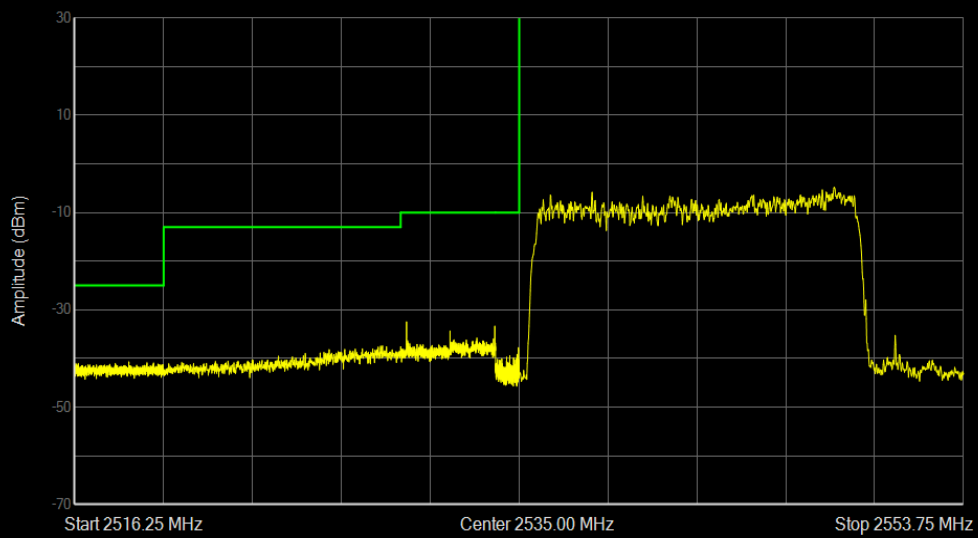
Band41 16QAM BW=15MHz Channel=40115 RB Size=75 Position=#0
