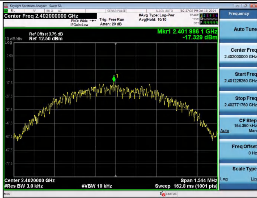
Power_Spectral_Density_NVNT_ANT1_1Mbps_2402
