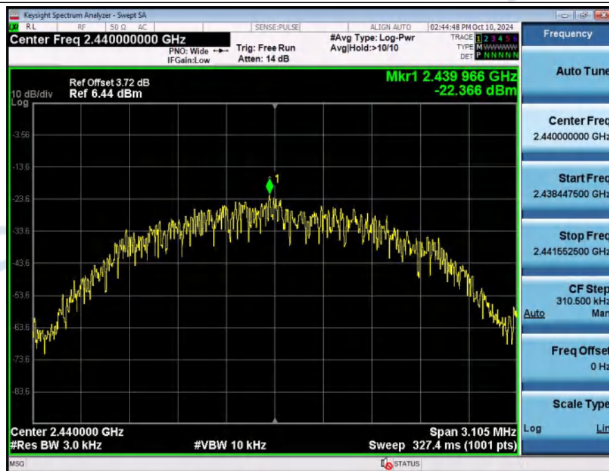
Power_Spectral_Density_NVNT_ANT1_2Mbps_2440
