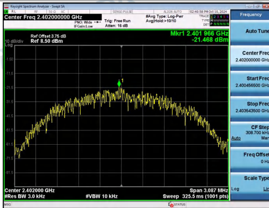
Power_Spectral_Density_NVNT_ANT1_2Mbps_2402
