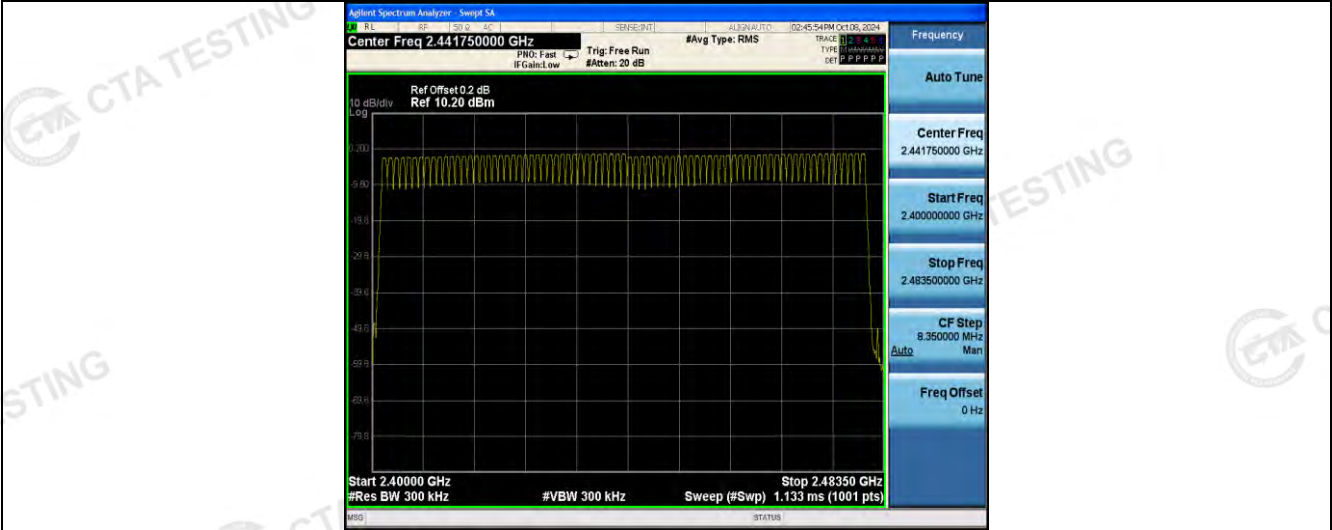
GFSK Modulation
