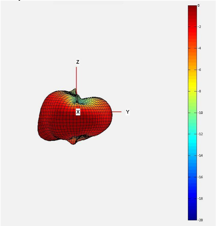
315MHz Y-Z plane
