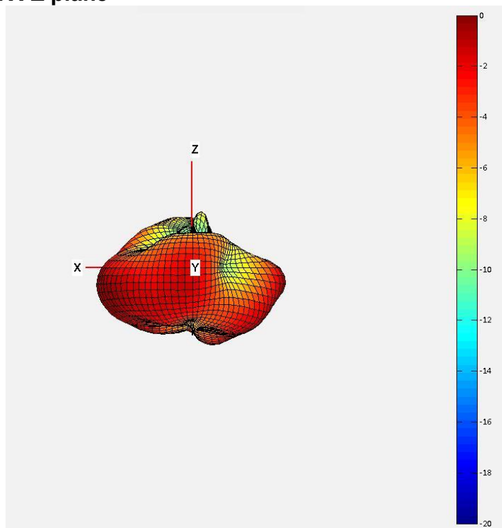
315MHz X-Z plane
