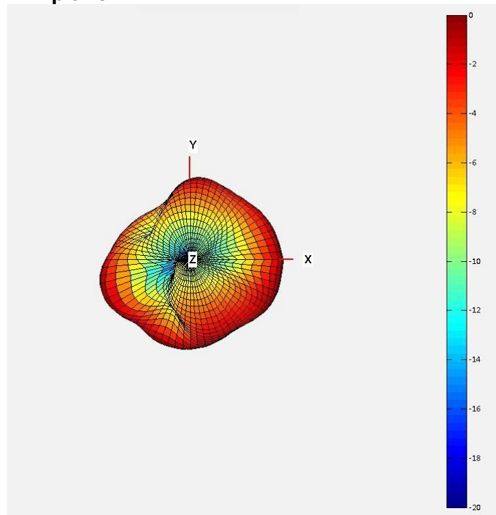
315MHz X-Y plane
