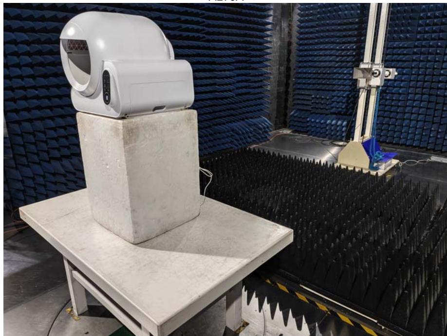
For Above 1GHz Test Site 1# AL70A
