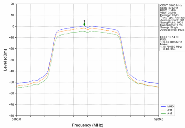
802.11ax(HEW20)_LCH_5180MHz_SU_/_MIMO_NTNV
