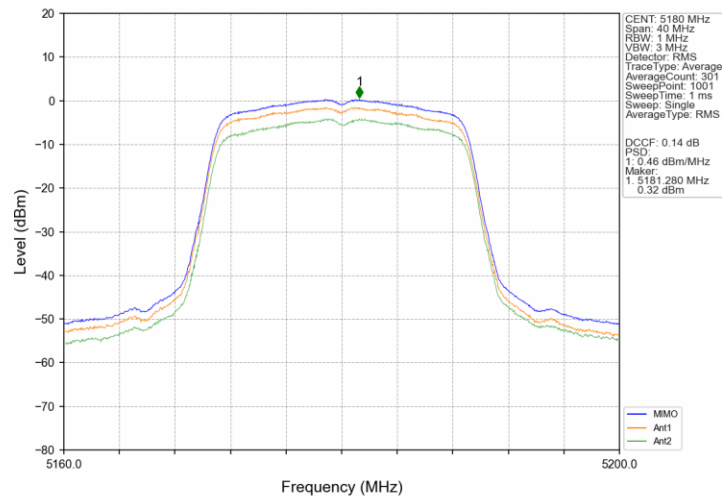
802.11ac(VHT20)_LCH_5180MHz_MIMO_NTNV
