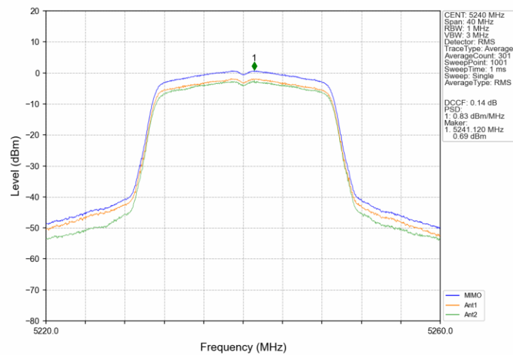
802.11ax(HEW20)_HCH_5240MHz_SU_/_MIMO_NTNV
