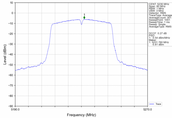
802.11ac(VHT40)_HCH_5230MHz_MIMO_NTNV
