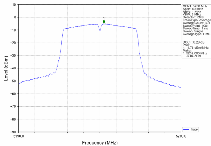
802.11ax(HEW40)_HCH_5230MHz_SU_/_Ant1_NTNV
