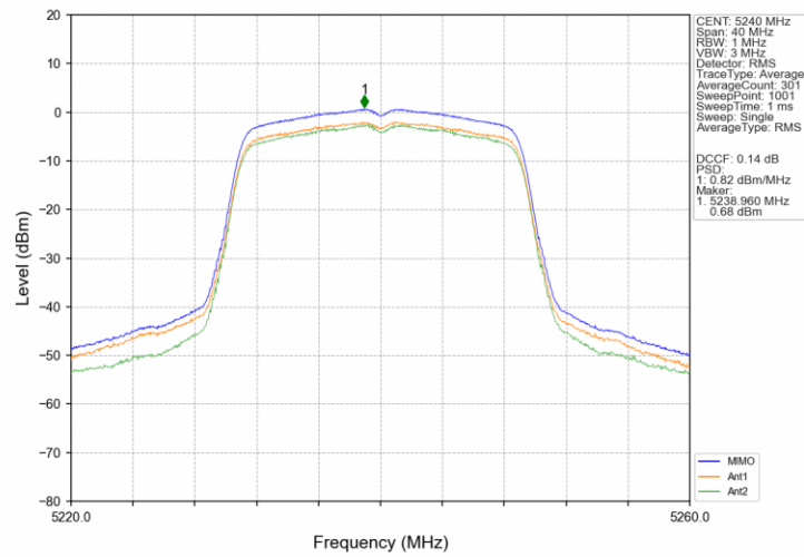
802.11ac(VHT20)_HCH_5240MHz_MIMO_NTNV
