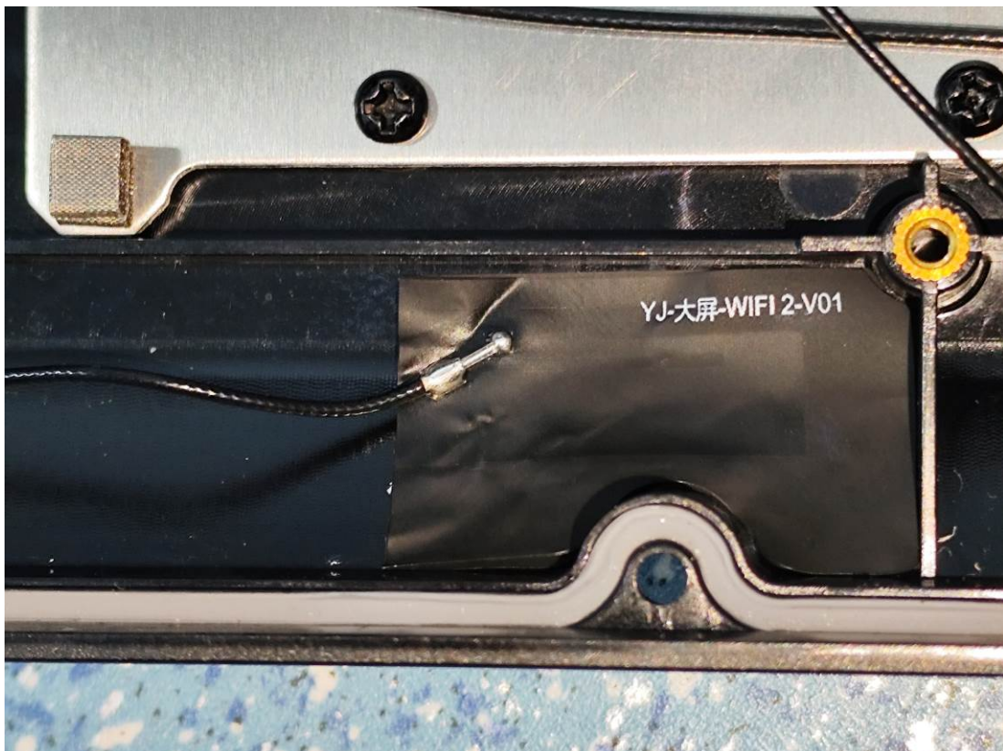
WIFI Antenna 2(Chain 1)
