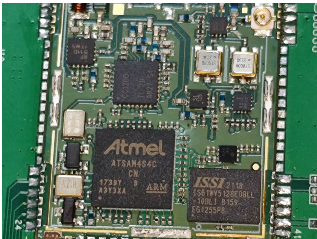
PMR Module (only RX) Unshielded
