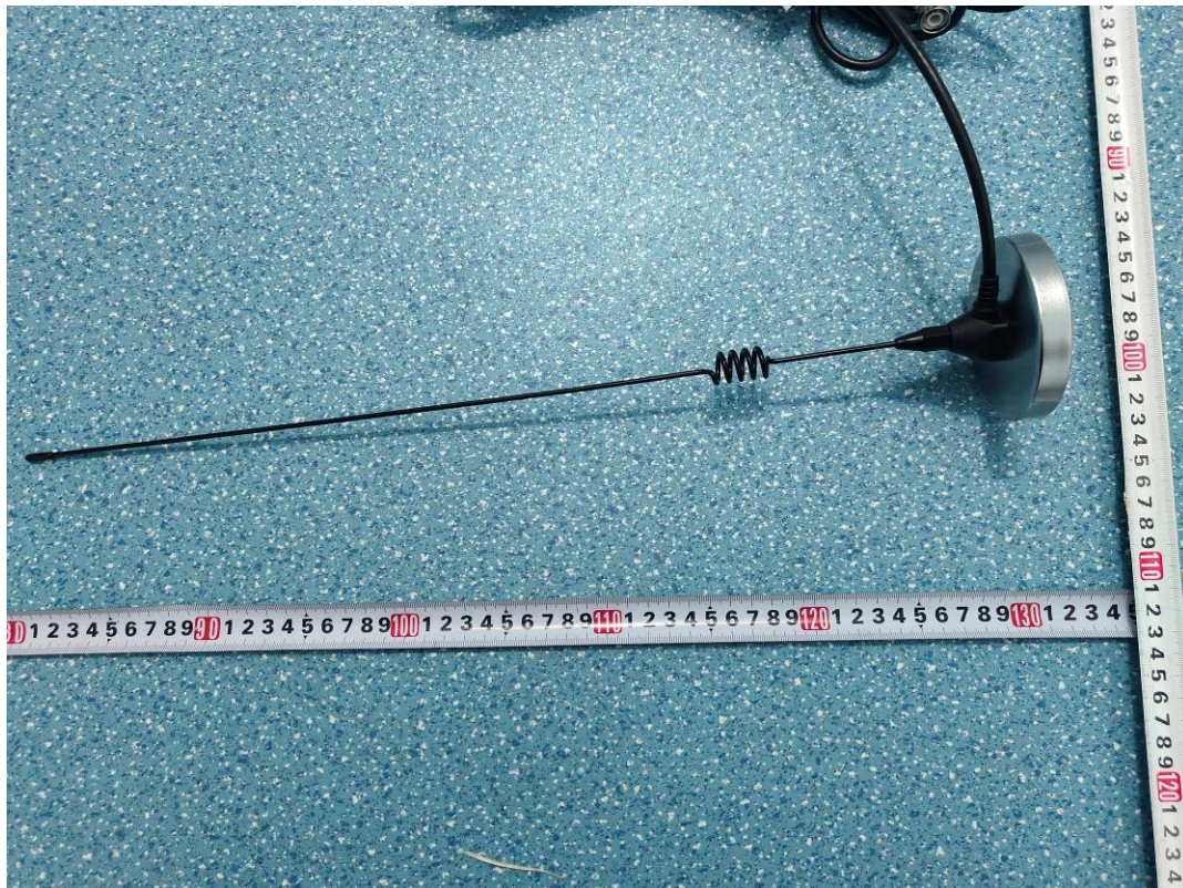
Radio Antenna (902-928MHz, only RX)
