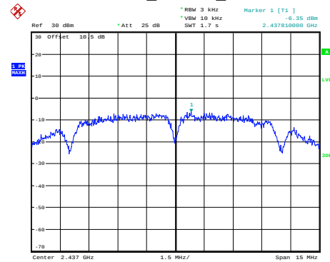
802.11b_Chain 1_2437MHz
