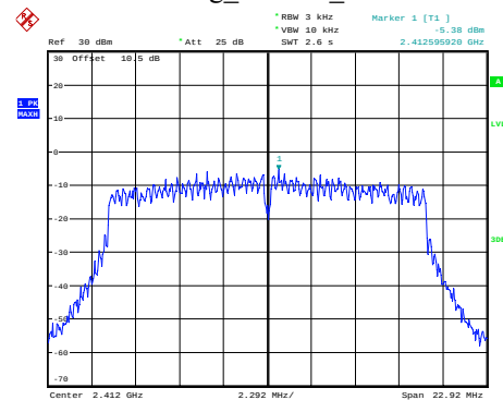
802.11g_Chain 1_2412MHz
