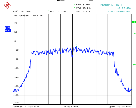
802.11g_Chain 1_2462MHz
