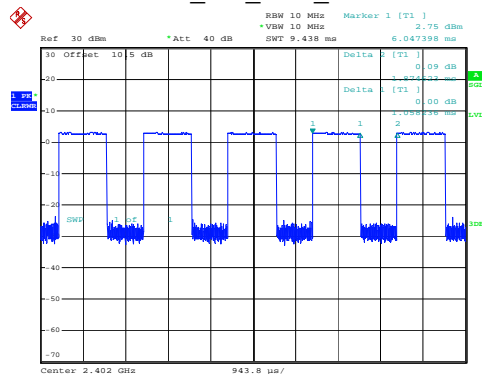
BLE_2M_Low_Channel
