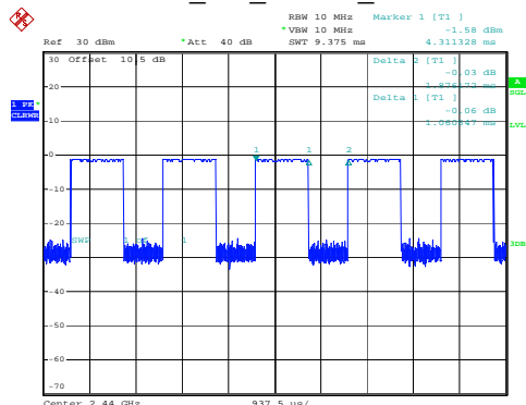
BLE_2M_Middle_Channel
