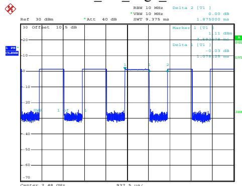
BLE_2M_High_Channel
