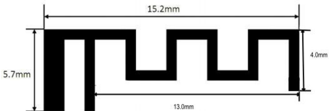
EUT Photo (Antenna Type: PCB ANT)
