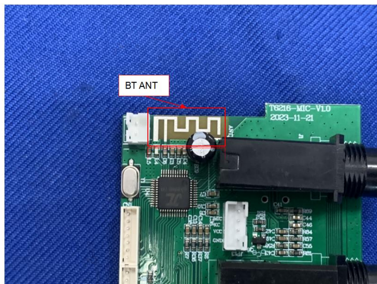
EUT Photo (Antenna Type: PCB ANT)
