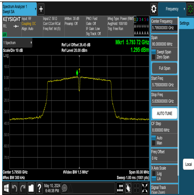
11N40MIMO-Ant3-5795-PASS
