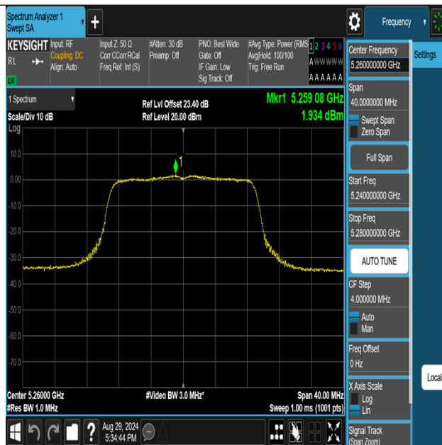
11AC20MIMO-Ant1-5260-PASS
