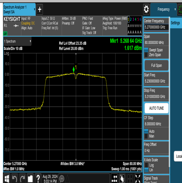
11N40MIMO-Ant2-5270-PASS
