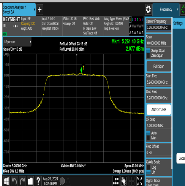
11AC20MIMO-Ant2-5260-PASS
