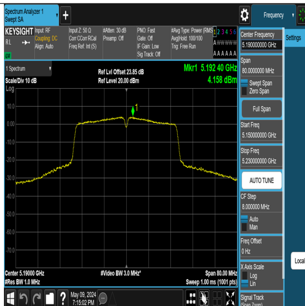
11N40MIMO-Ant3-5190-PASS
