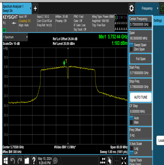
11N40MIMO-Ant3-5755-PASS
