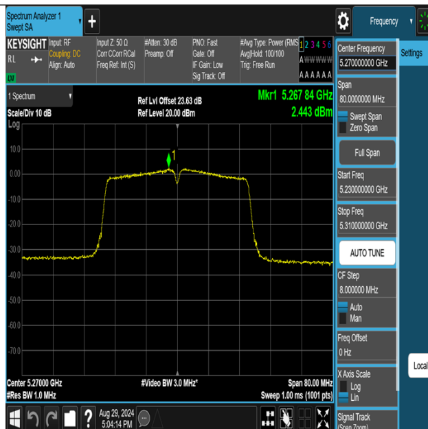
11N40MIMO-Ant3-5270-PASS
