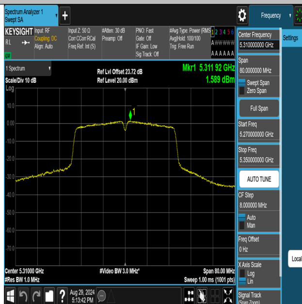
11N40MIMO-Ant1-5310-PASS
