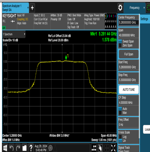
11AC20MIMO-Ant1-5280-PASS
