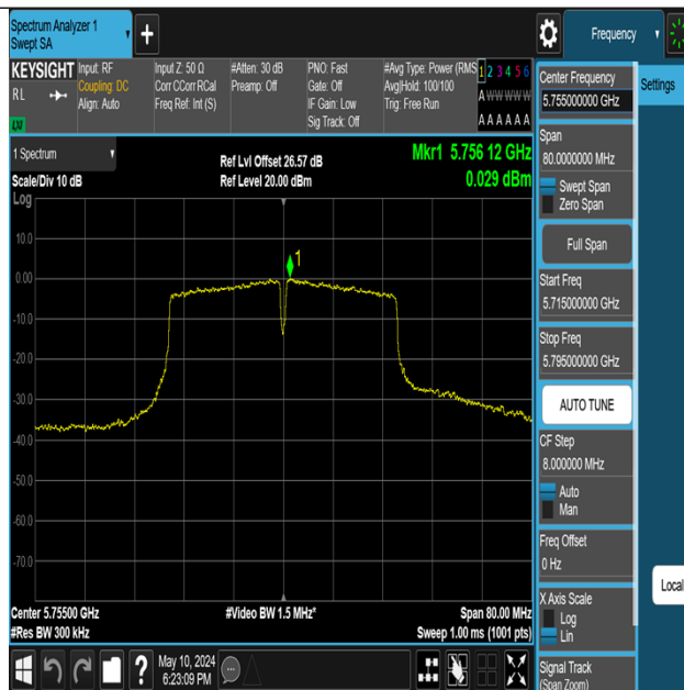
11N40MIMO-Ant2-5755-PASS
