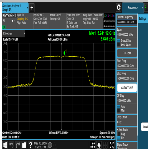
11AC20MIMO-Ant3-5240-PASS
