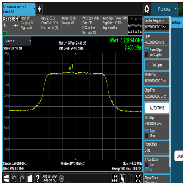
11AC20MIMO-Ant3-5260-PASS
