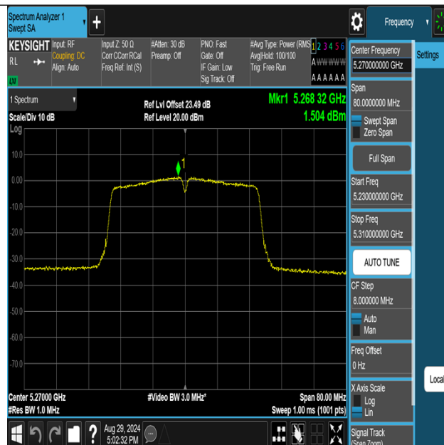
11N40MIMO-Ant1-5270-PASS
