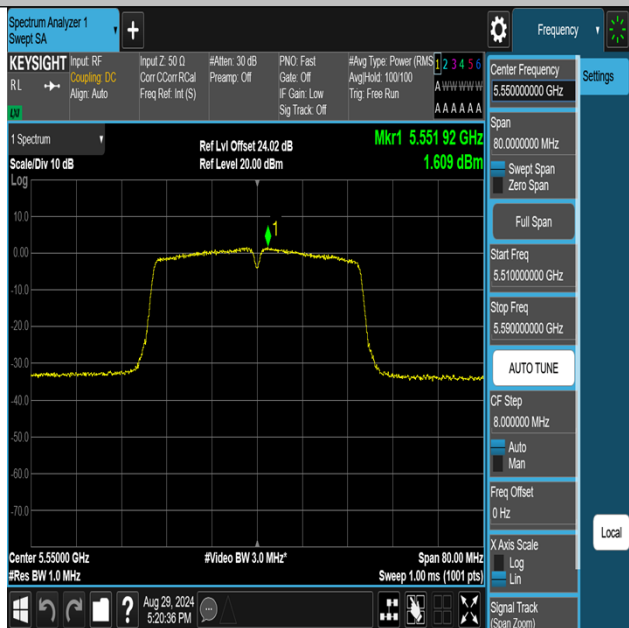
11N40MIMO-Ant1-5550-PASS
