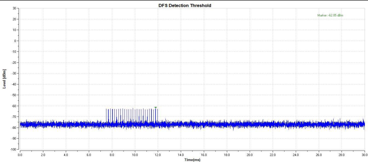
11AC20-5260-Type2-PASS
