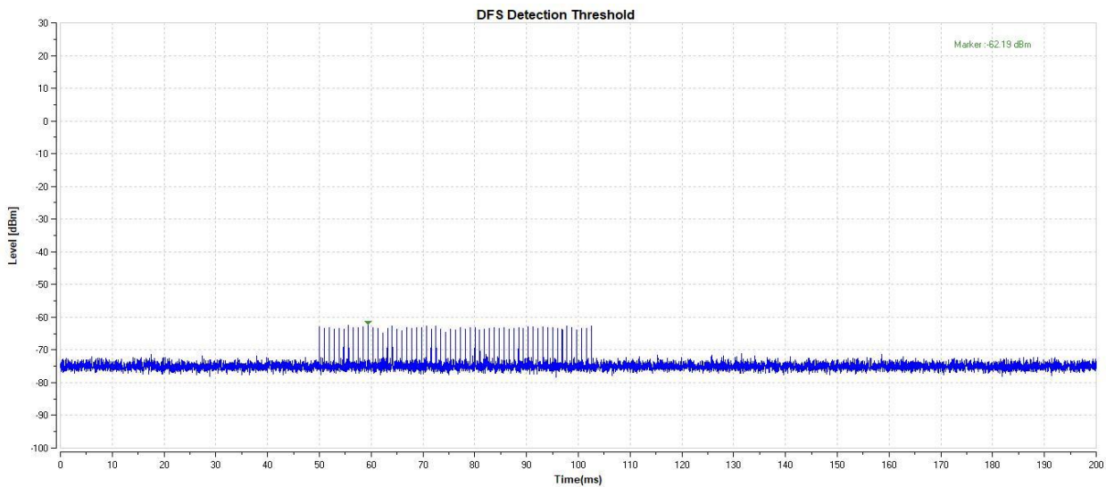
11AC20-5260-Type1-PASS
