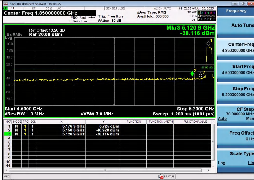
11A-Ant2-5180-PASS
