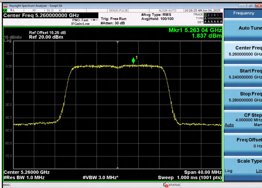
11N20SISO-Ant2-5260-PASS
