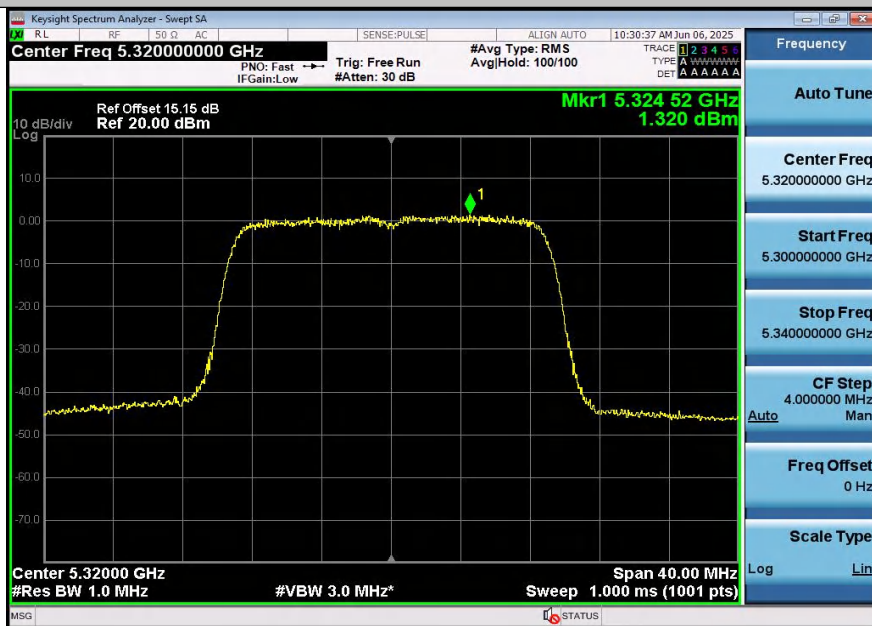
11N20SISO-Ant2-5320-PASS
