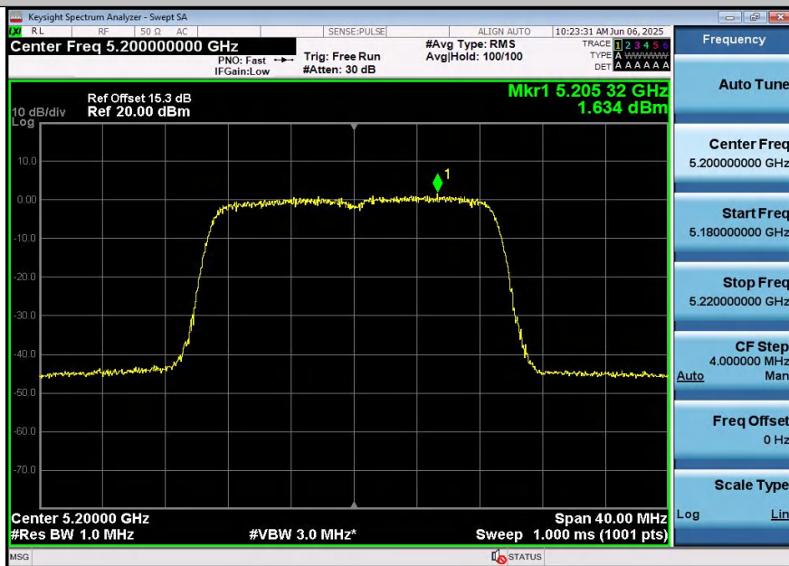
11N20SISO-Ant2-5200-PASS
