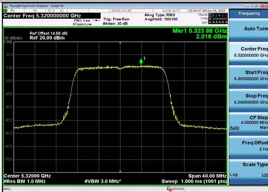
11A-Ant2-5320-PASS
