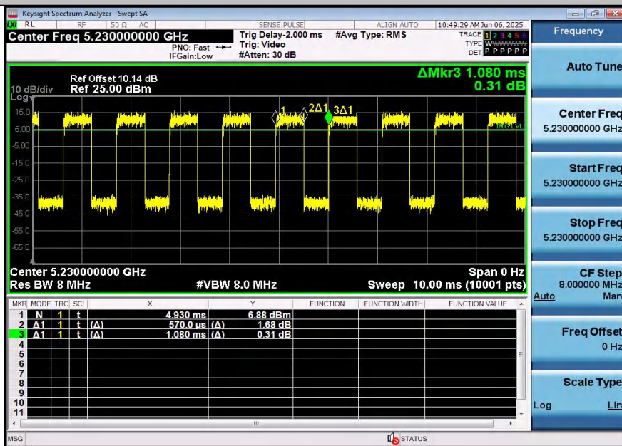
NTNV-11N40SISO-Ant2-5230
