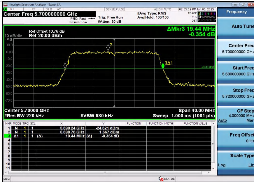
11N20SISO-Ant1-5700
