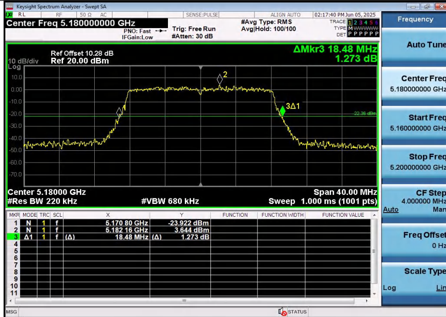
11A-Ant1-5180
