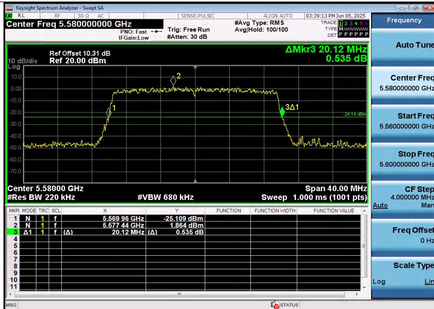
11AC20SISO-Ant1-5580
