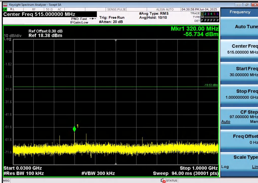
11B-Ant2-2412-30~1000-PASS
