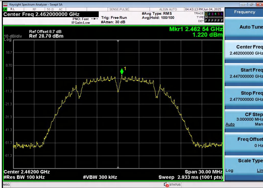
11B-Ant2-2462-0~Reference-PASS
