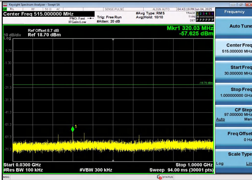
11B-Ant2-2462-30~1000-PASS
