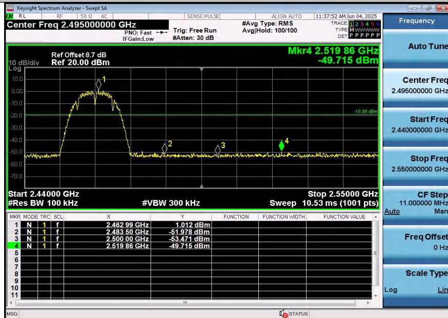
11B-Ant1-2462-PASS
