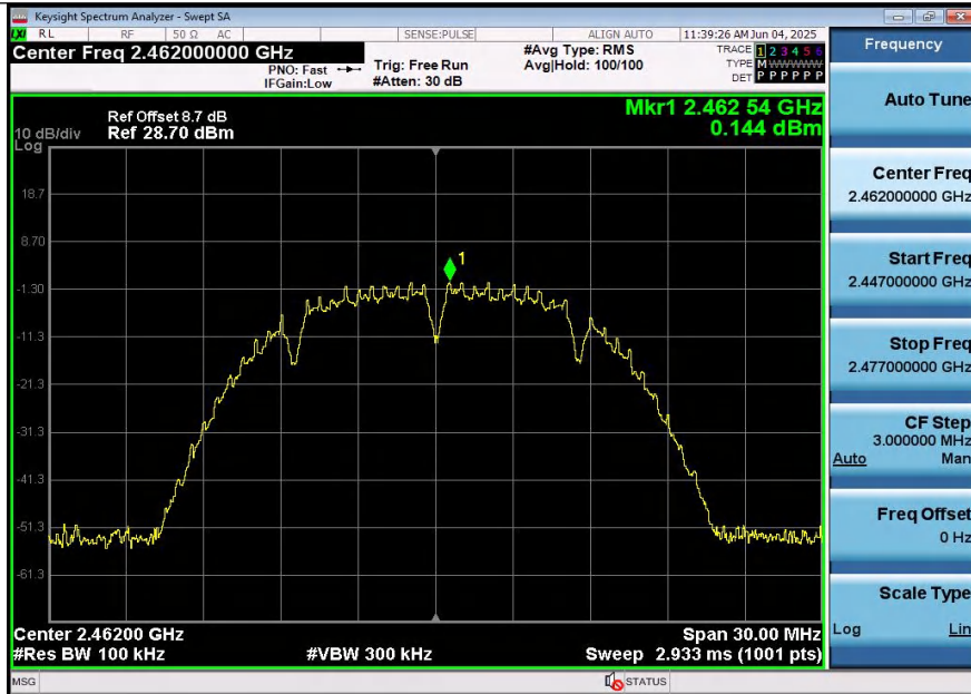
11B-Ant1-2462-0~Reference-PASS
