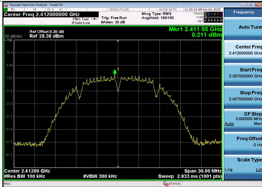
11B-Ant1-2412-0~Reference-PASS
