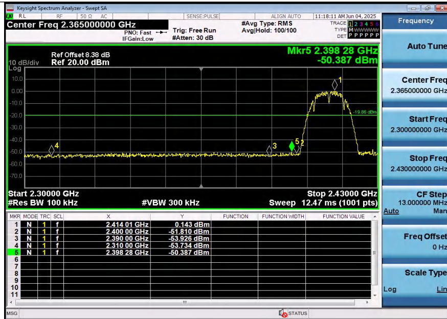
11B-Ant1-2412-PASS
