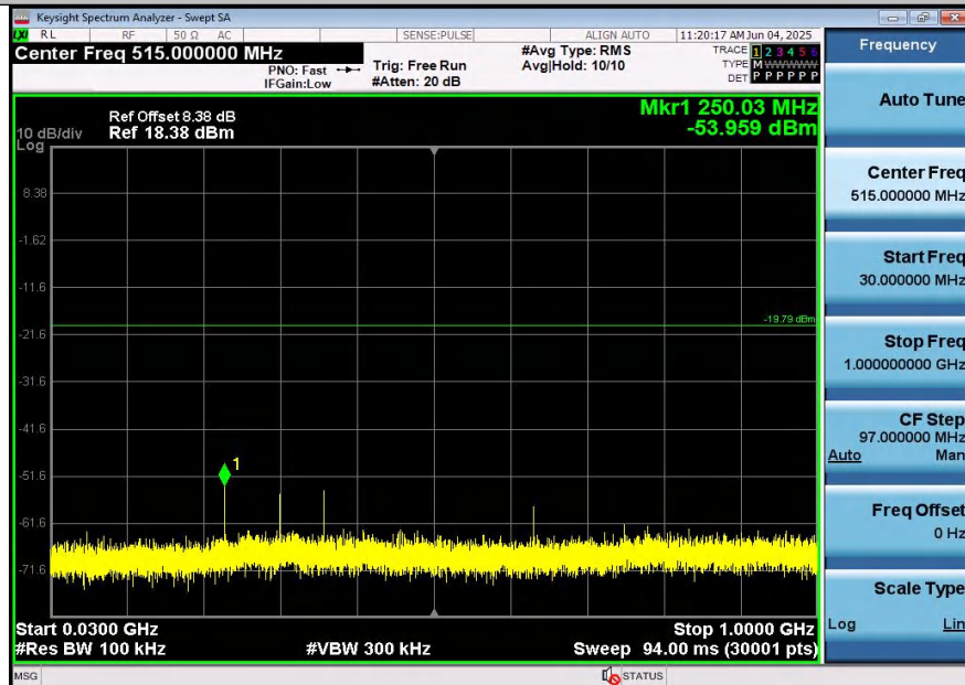
11B-Ant1-2412-30~1000-PASS
