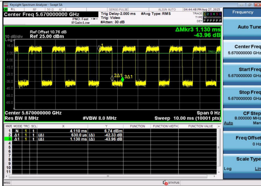
NTNV-11N40SISO-Ant1-5670
