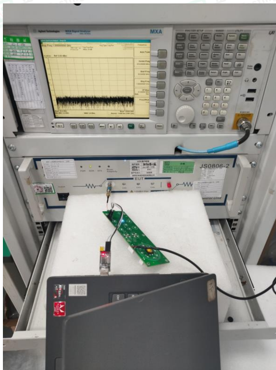
Test Setup Photo of Line RF Conducted Measurement
